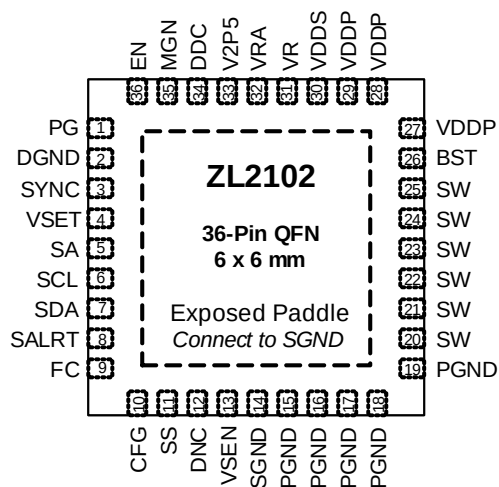
ZL2102 (36 LD 6X6 QFN) TOP VIEW
