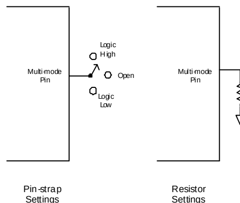
FIGURE 11. PIN-STRAP AND RESISTOR SETTING EXAMPLES
