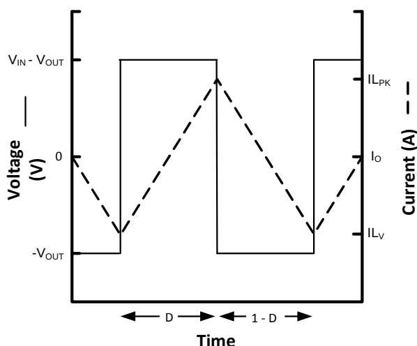
FIGURE 9. OUTPUT CURRENT
