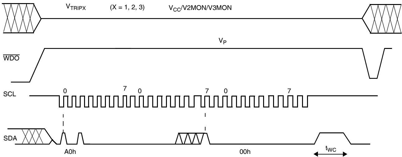
Figure 4. Watchdog Restart
