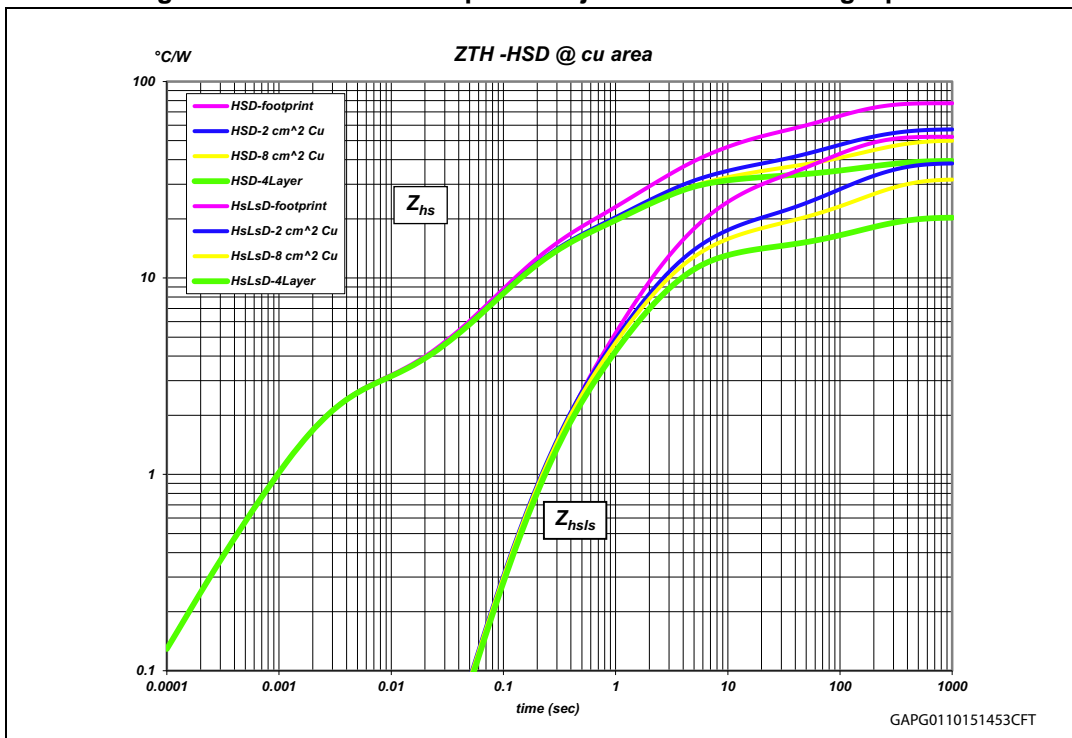
Figure 25. HSD thermal impedance junction ambient single pulse
