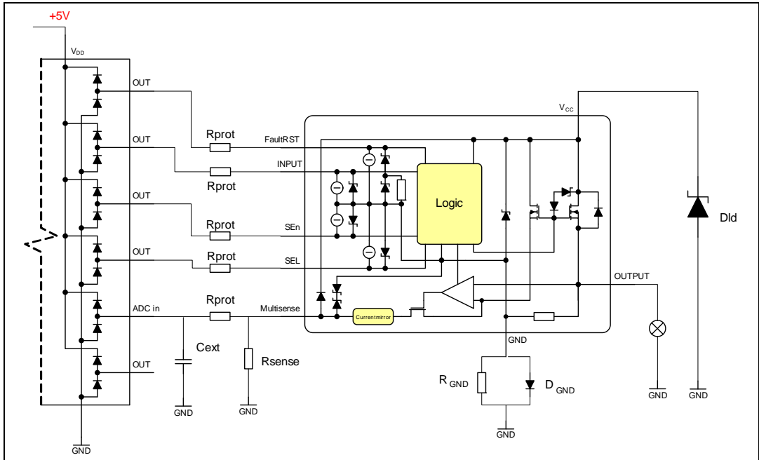
Figure 35. Application diagram
