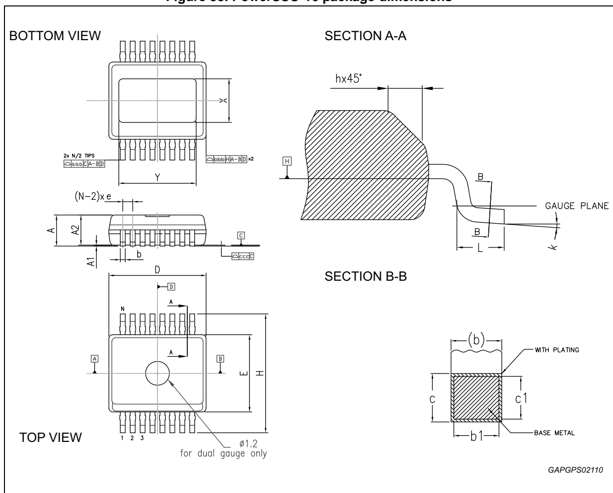
Figure 53. PowerSSO-16 package dimensions
