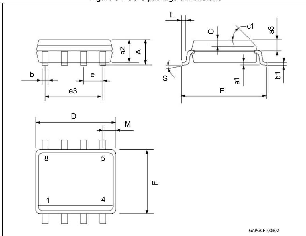
Figure 54. SO-8 package dimensions
