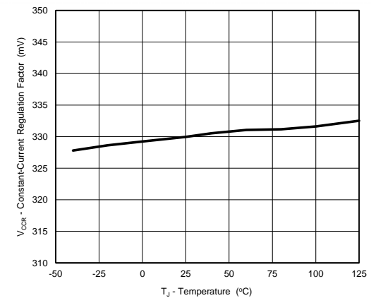
Figure 6. Constant-Current Regulation Factor vs. Temperature
