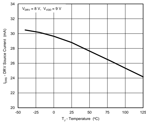
Figure 8. DRV Source Current vs. Temperature
