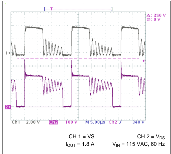
Figure 20. Switching Waveform
