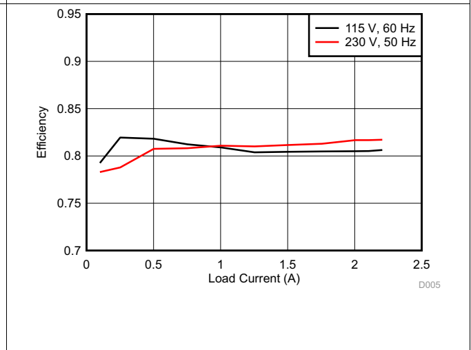
Figure 22. Efficiency
