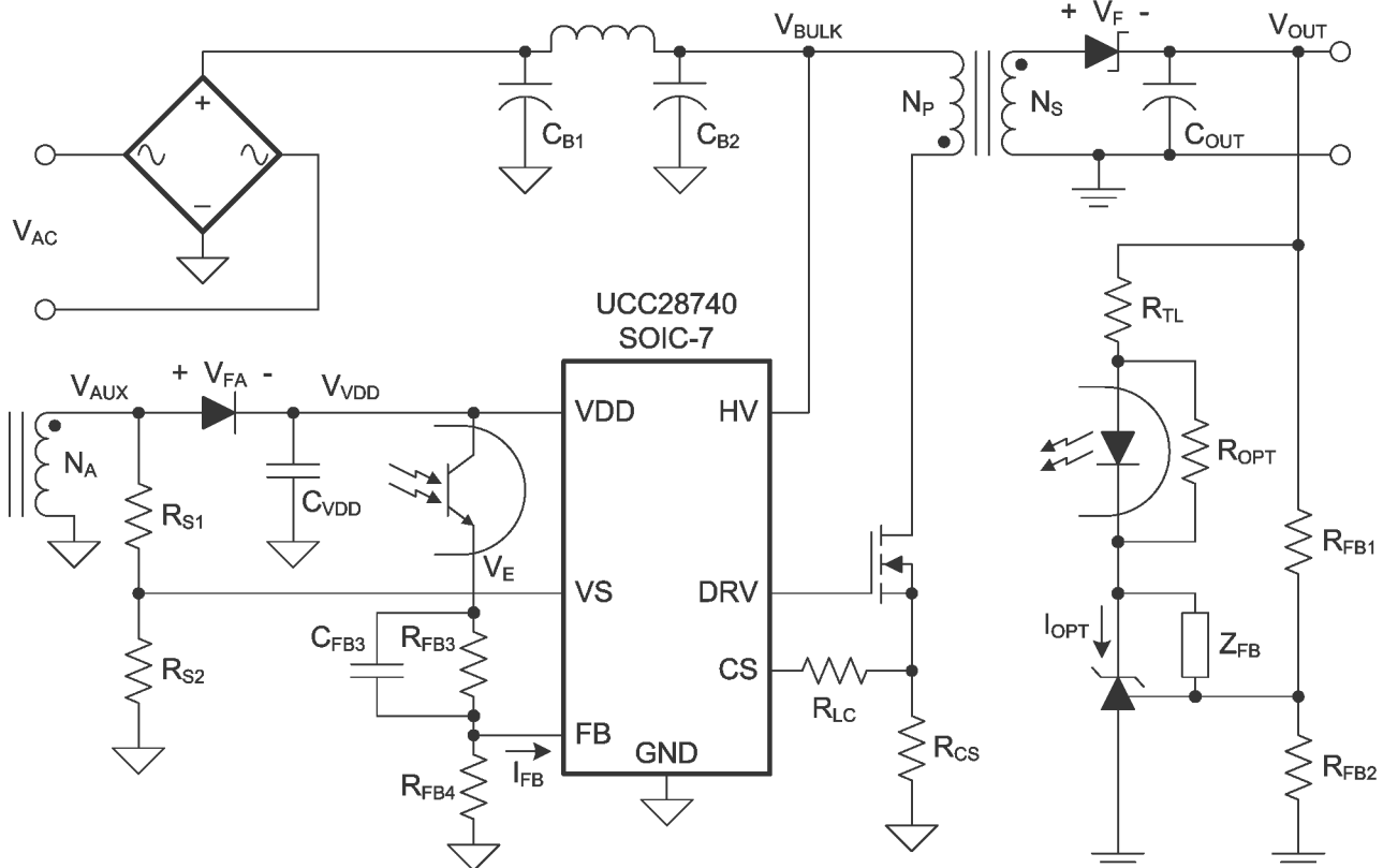
Figure 18. Design Procedure Application Example
