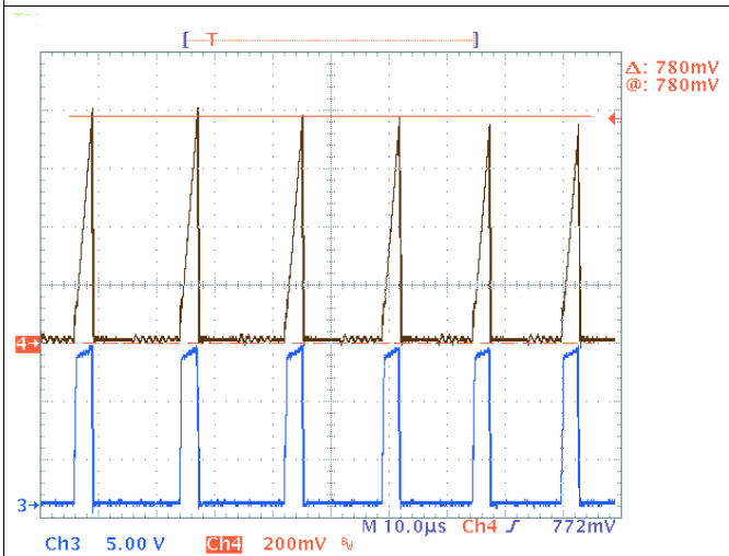
Figure 21. EMI Dithering
