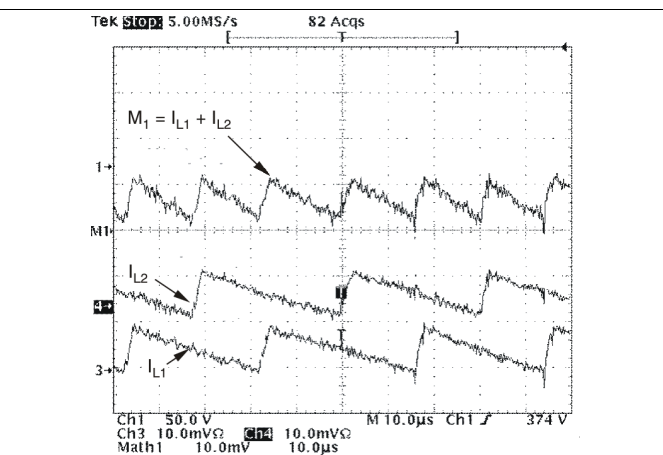
图 36. Inductor and Input Ripple Current at 265 V_{RMS} Input at Peak Line Voltage
