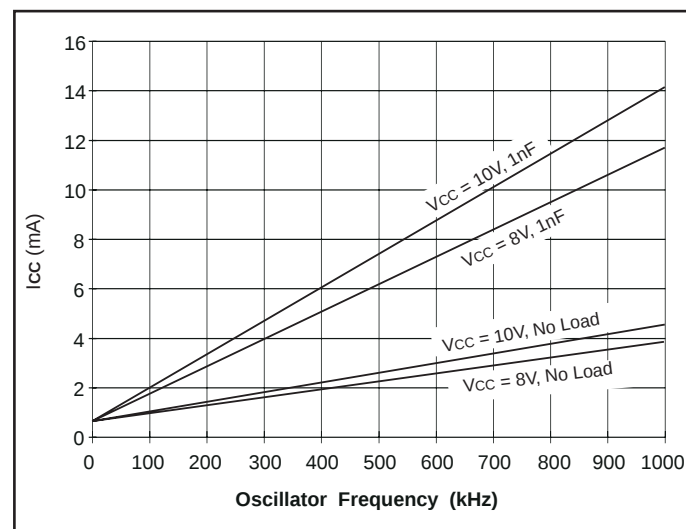
Figure 8. UCC1800 I_{CC} vs. oscillator frequency.
