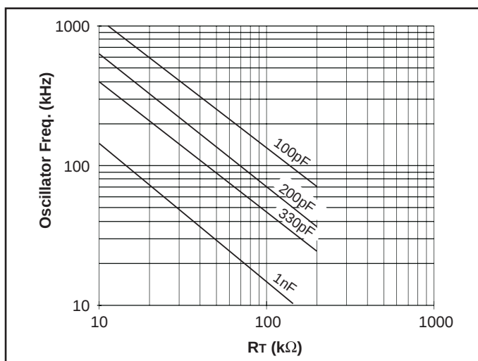
Figure 4. UCC1800/1/2/4 oscillator frequency vs. R_T and C_T .
