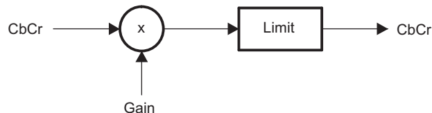
Figure 2-11. CbCr Component Gain, Offset, Limit
