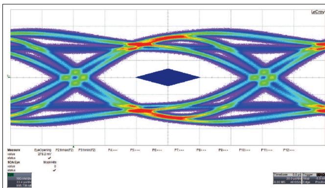
图 33. SuperSpeed TX Eye for Downstream Port 1
