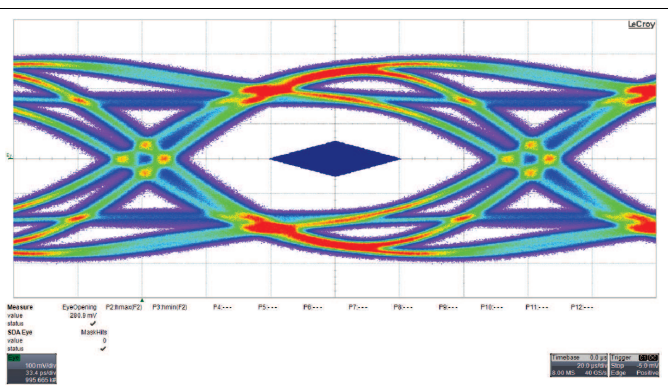
图 34. SuperSpeed TX Eye for Downstream Port 2
