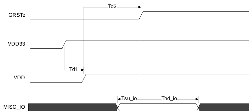
图 1. Power-Up Timing Requirements
