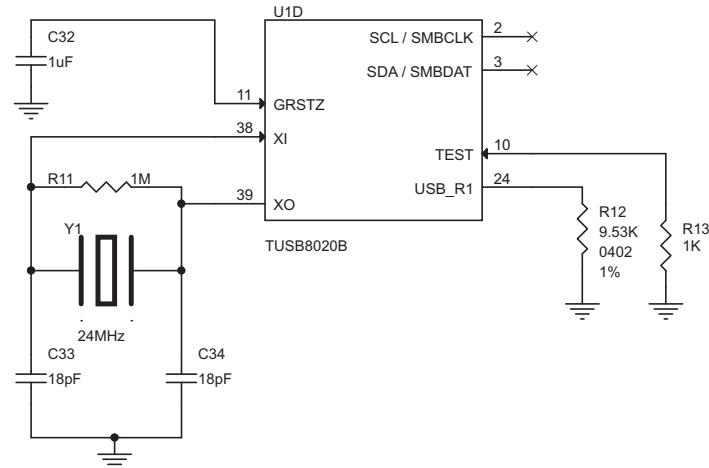
图 31. Clock, Reset, and Miscellaneous
