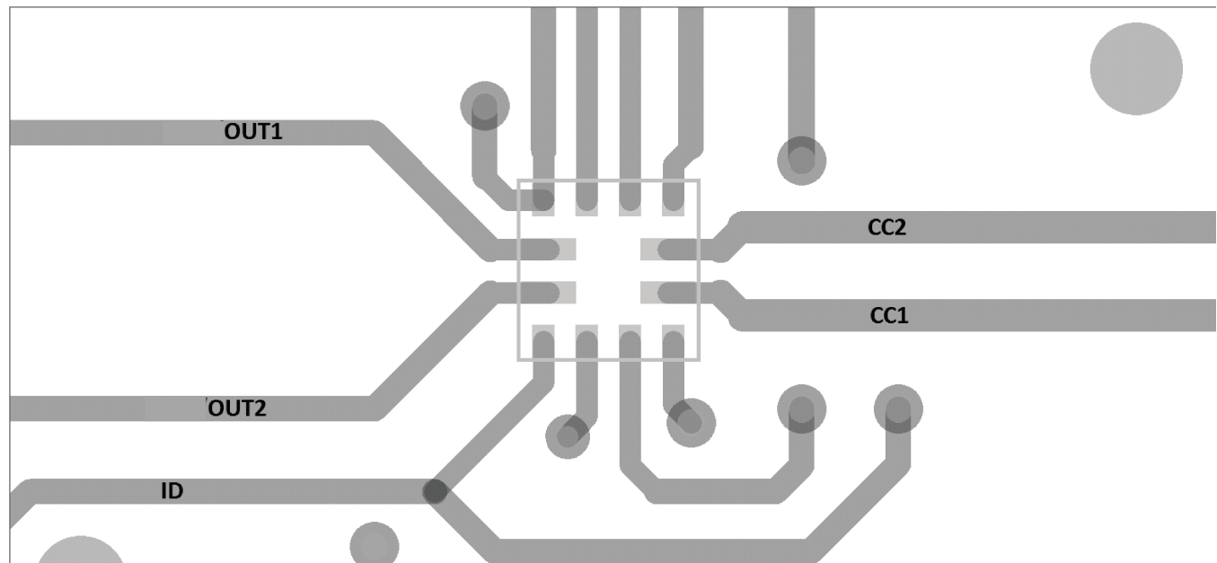
Figure 5. TUSB321AI Layout
