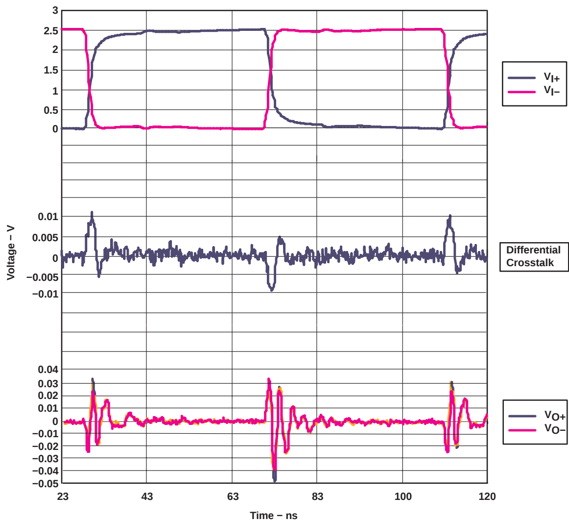
Figure 6. Differential Crosstalk
