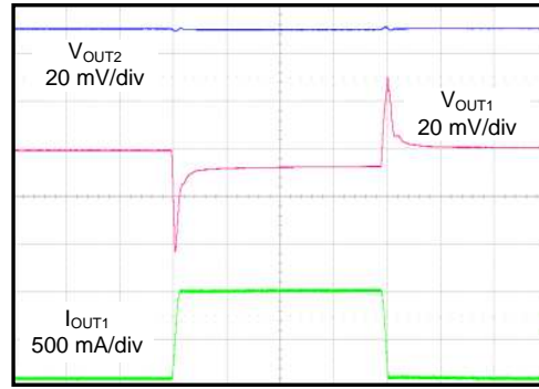
V_{\text{INX}} = 5.5\text{ V} , I_{\text{OUTX}} = 100\text{ mA to }1\text{ A to }100\text{ mA} at 1\text{ A}/\mu\text{s} , C_{\text{OUTX}} = 10\text{ }\mu\text{F}
