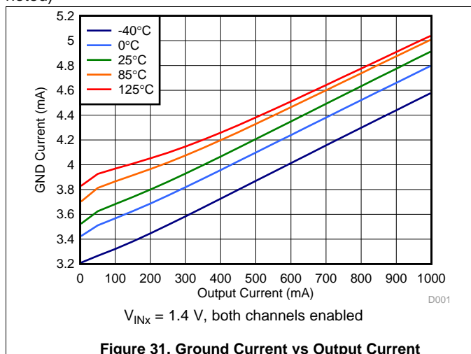
Figure 31. Ground Current vs Output Current
