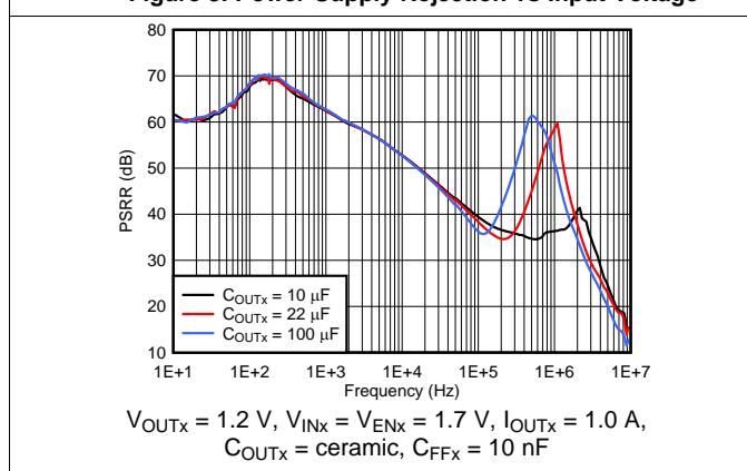
Figure 5. Power-Supply Rejection vs Output Capacitance
