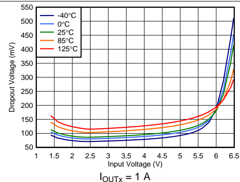
Figure 24. Dropout Voltage vs Input Voltage
