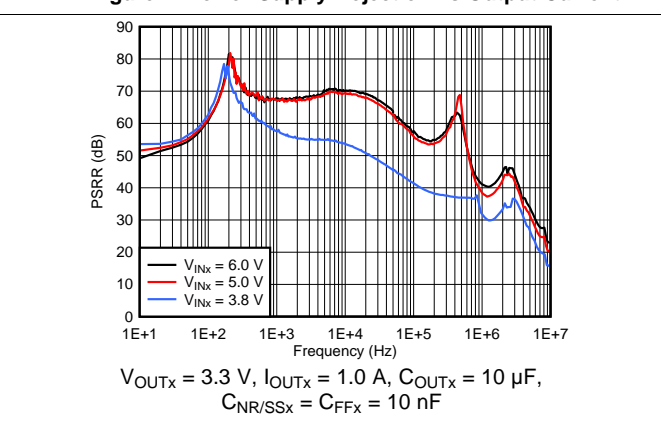
Figure 6. Power-Supply Rejection vs Input Voltage
