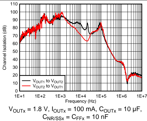
Figure 7. Channel-to-Channel Output Voltage Isolation vs Frequency
