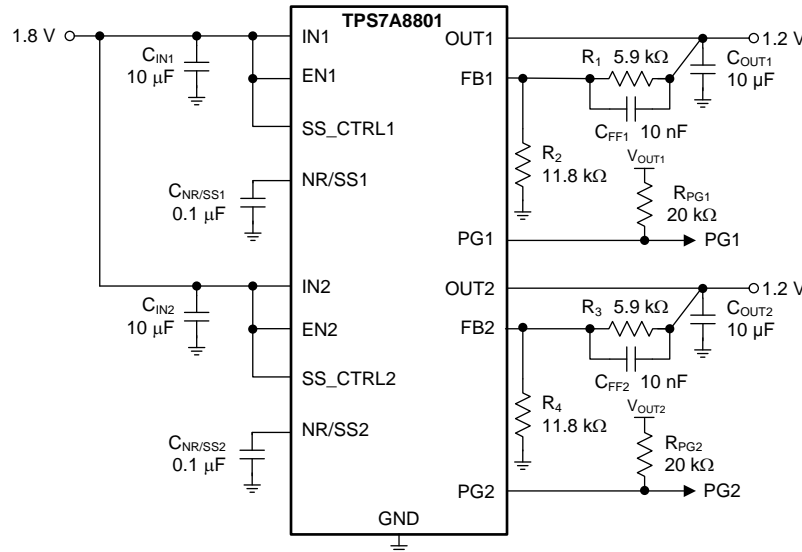
Figure 43. Application Example
