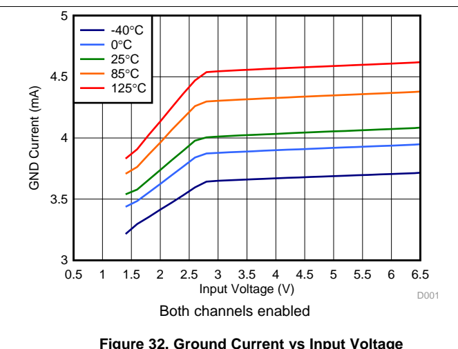
Figure 32. Ground Current vs Input Voltage
