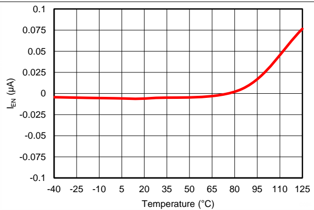
Figure 34. Minimum ANY-OUT V_{OUT} , Maximum V_{IN} Enable Current vs Temperature V_{OUT(TARGET)} = 0.8\text{ V} , V_{IN} = V_{EN} = 6.5\text{ V} , V_{BIAS} = \text{Open}
