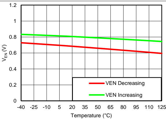
Figure 33. Minimum ANY-OUT V_{OUT} , Maximum V_{IN} Enable Threshold vs Temperature V_{OUT(TARGET)} = 0.8\text{ V} , V_{IN} = 6.5\text{ V} , V_{BIAS} = \text{Open}
