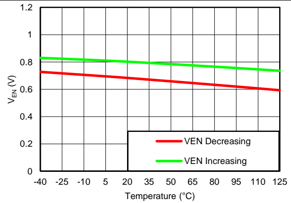
Figure 32. Minimum ANY-OUT V_{OUT} , Minimum V_{IN} , No BIAS Enable Threshold vs Temperature V_{OUT(TARGET)} = 0.8\text{ V} , V_{IN} = 1.4\text{ V} , V_{BIAS} = \text{Open}
