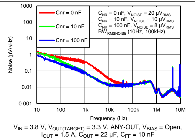
Figure 44. Spectral Noise Density vs C_{NR/SS}
