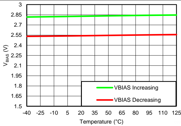
Figure 31. Minimum ANY-OUT V_{OUT} , Minimum V_{IN} BIAS UVLO Threshold vs Temperature V_{OUT(TARGET)} = 0.8\text{ V} , V_{IN} = 1.1\text{ V}
