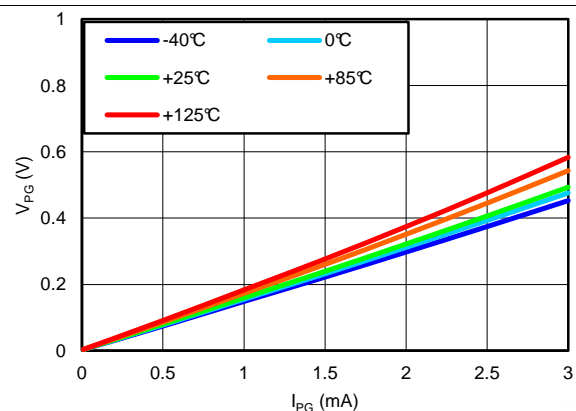
Figure 36. Minimum ANY-OUT V_{OUT} , Minimum V_{IN} , No BIAS PG Low Voltage vs PG Current V_{OUT(TARGET)} = 0.8\text{ V} , V_{IN} = 1.4\text{ V} , V_{BIAS} = \text{Open}
