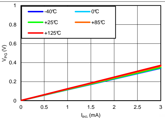
Figure 35. Minimum ANY-OUT V_{OUT} , Maximum V_{IN} , No BIAS PG Low Voltage vs PG Current V_{IN} = 6.5\text{ V} , V_{OUT(TARGET)} = 0.8\text{ V} , V_{BIAS} = \text{Open}
