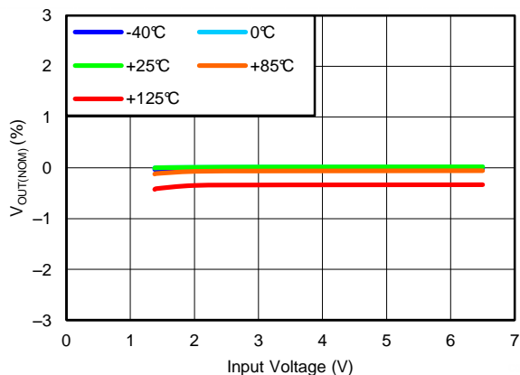
Figure 2. LINE REGULATION ( V_{OUT(TARGET)} = 0.8\text{ V} , ANY-OUT, I_{OUT} = 5\text{ mA} , V_{BIAS} = \text{Open} )
