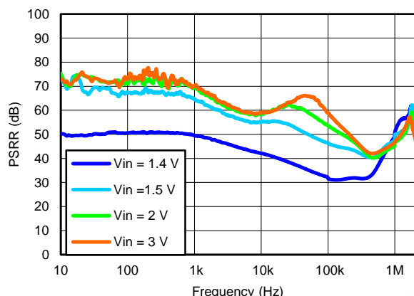
Figure 43. POWER-SUPPLY REJECTION vs INPUT VOLTAGE ( V_{OUT(TARGET)} = 3.3\text{ V} , ANY-OUT, V_{BIAS} = \text{Open} , I_{OUT} = 1.5\text{ A} , C_{OUT} = 22\ \mu\text{F} , C_{NR/SS} = C_{FF} = 10\text{ nF} )
