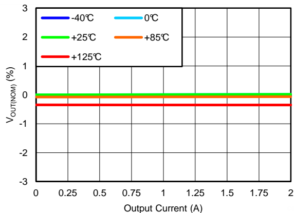
Figure 7. LOAD REGULATION ( V_{OUT(TARGET)} = 0.8\text{ V} , ANY-OUT, V_{IN} = 1.1\text{ V} , V_{BIAS} = 3\text{ V} )
