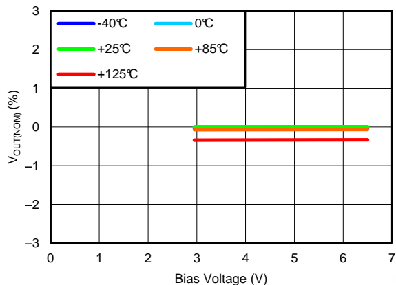
Figure 6. BIAS LINE REGULATION ( V_{OUT(TARGET)} = 0.8\text{ V} , ANY-OUT, V_{IN} = 1.1\text{ V} , I_{OUT} = 5\text{ mA} )
