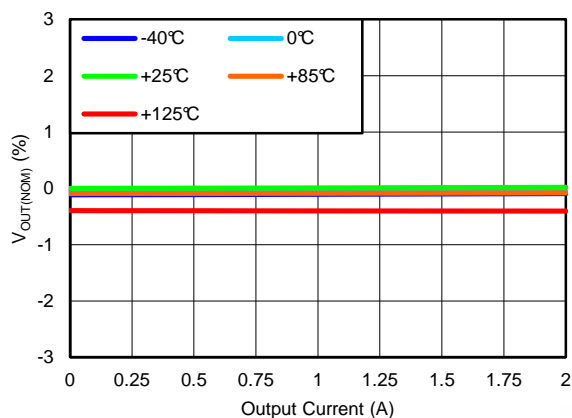
Figure 5. LOAD REGULATION ( V_{OUT(TARGET)} = 3.95\text{ V} , ANY-OUT, V_{IN} = 4.25\text{ V} , V_{BIAS} = \text{Open} )
