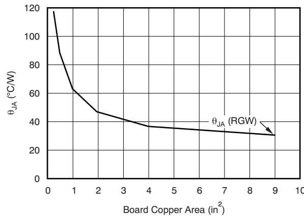
Figure 53. θ JA vs Board Size
