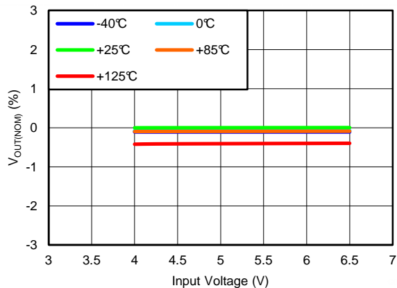
Figure 3. LINE REGULATION ( V_{OUT(TARGET)} = 3.95\text{ V} , ANY-OUT, I_{OUT} = 5\text{ mA} , V_{BIAS} = \text{Open} )
