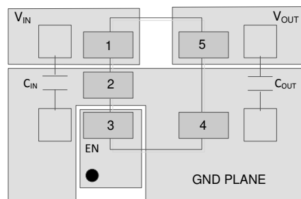
图 10-1. Adjustable Version Layout Example
