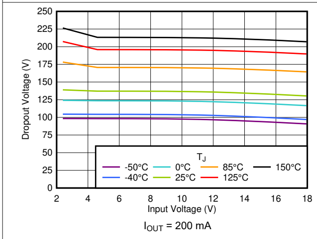
图 6-5. Dropout Voltage vs V_{IN}
