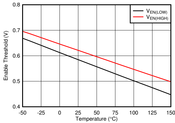
图 6-13. V_{EN} vs Temperature
