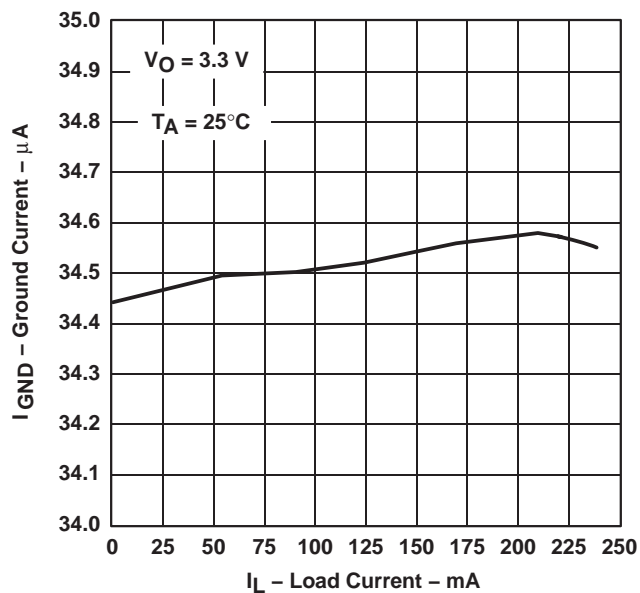
TPS76633 GROUND CURRENT vs LOAD CURRENT
