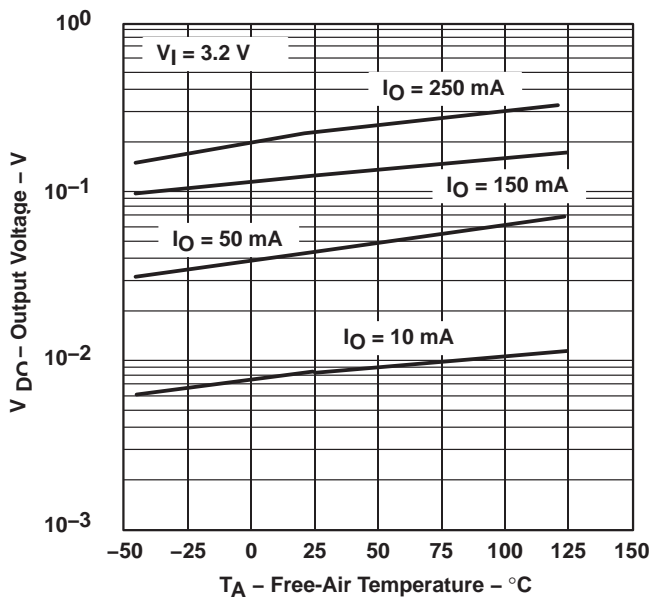
TPS76633 DROPOUT VOLTAGE vs FREE-AIR TEMPERATURE
