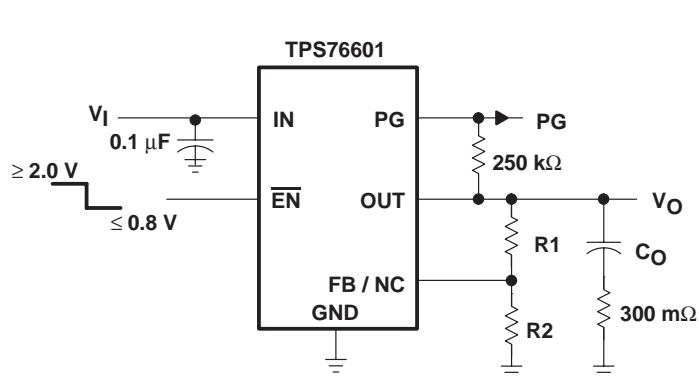
Figure 29. TPS76601 Adjustable LDO Regulator Programming
