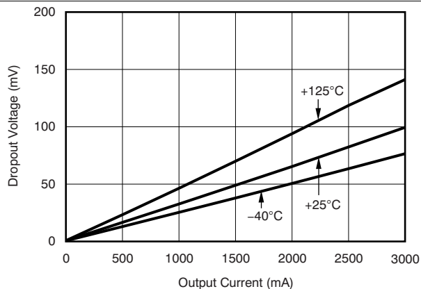
Figure 36. V_{IN} Dropout Voltage vs I_{OUT} and Temperature ( T_J )
