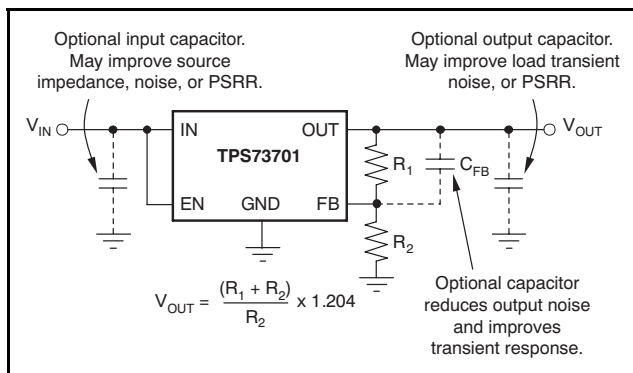
Figure 27. Typical Application Circuit for Adjustable-Voltage Version
