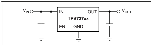
Figure 26. Typical Application Circuit for Fixed-Voltage Versions
