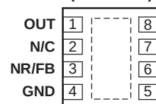
DRB PACKAGE 3mm x 3mm SON (TOP VIEW)
