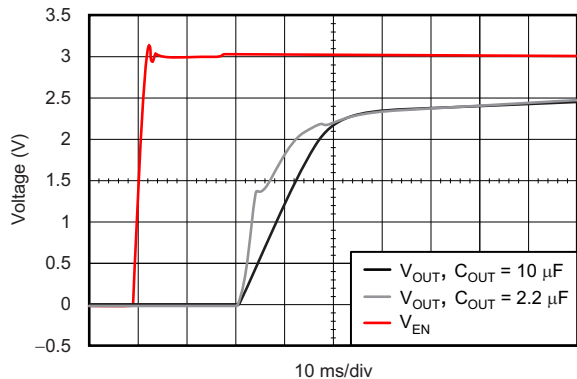
Figure 17. TPS73525 Turnon Response ( V_{IN} = V_{EN} )
