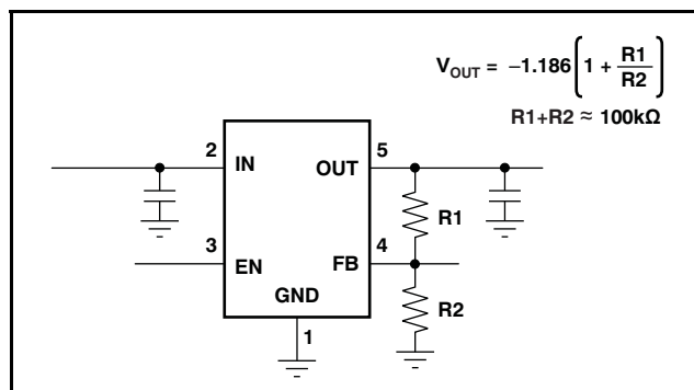
Figure 27. TPS72301 Adjustable LDO Regulator Programming
