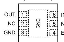
DRV PACKAGE 2-mm × 2-mm SON-6 (TOP VIEW)
