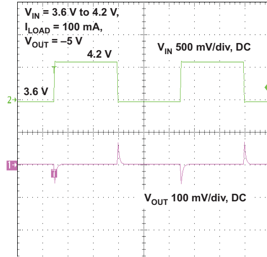
LINE TRANSIENT RESPONSE, -5 V
