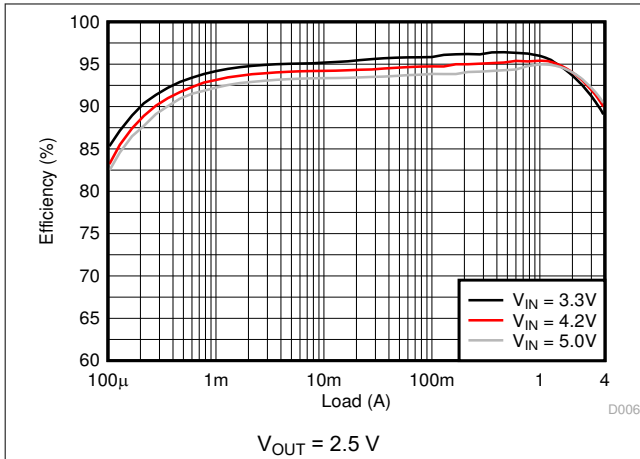
Figure 9-15. Efficiency
