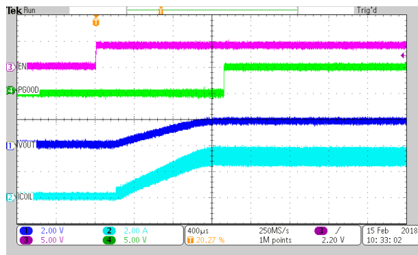
Load = 0.6 \Omega TPS62825 and TPS62826
