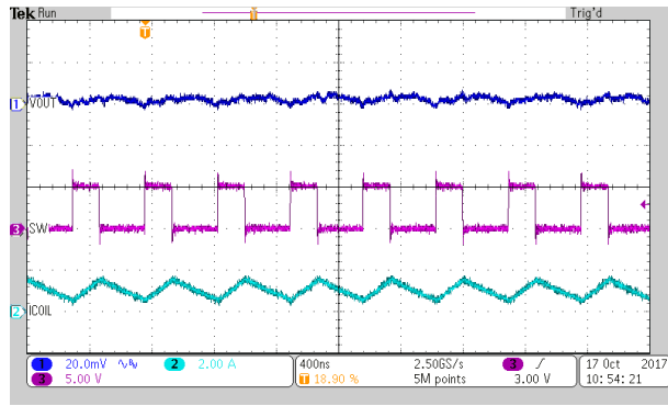
I_{OUT} = 1.0 \text{ A} TPS62825 and TPS62826
