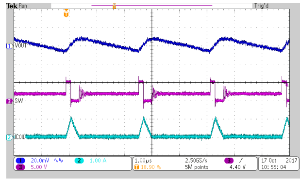
I_{OUT} = 0.1 \text{ A} TPS62825 and TPS62826
