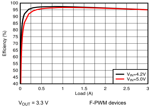
Figure 9-21. PWM Efficiency
