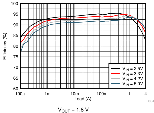
Figure 9-11. Efficiency
