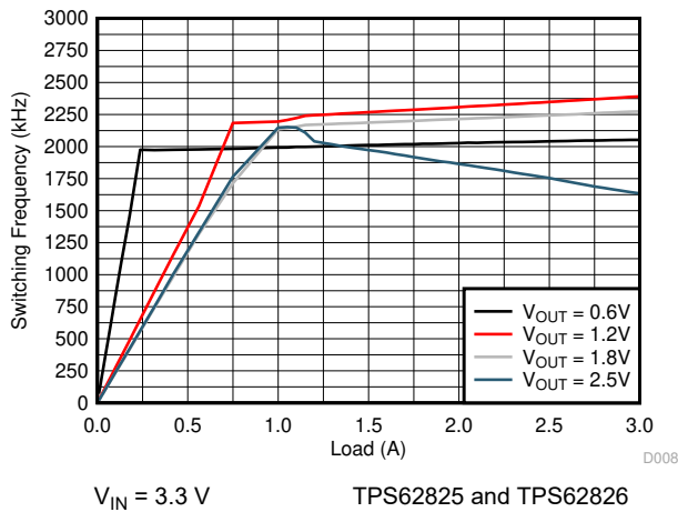
Figure 9-23. Switching Frequency
