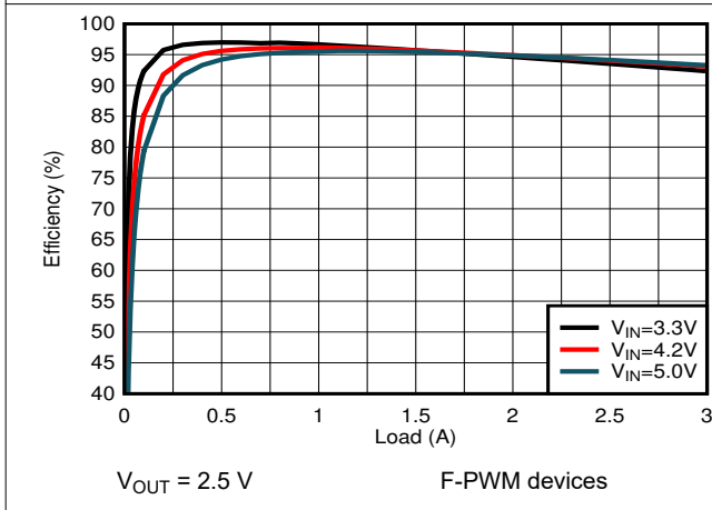
Figure 9-17. PWM Efficiency
