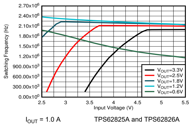
Figure 9-26. Switching Frequency
