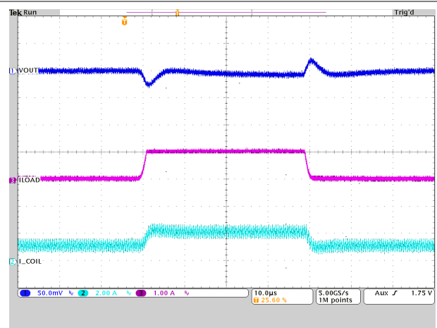
I_{OUT} = 1 \text{ A to } 2 \text{ A} TPS62825A and TPS62826A
