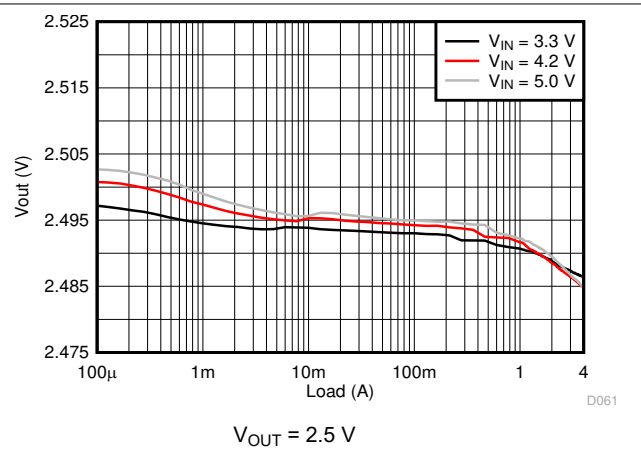
Figure 9-16. Load Regulation
