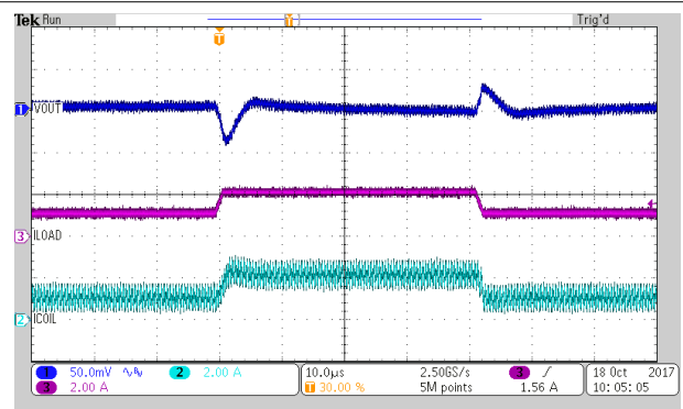
I_{OUT} = 1 \text{ A to } 2 \text{ A} TPS62825 and TPS62826
