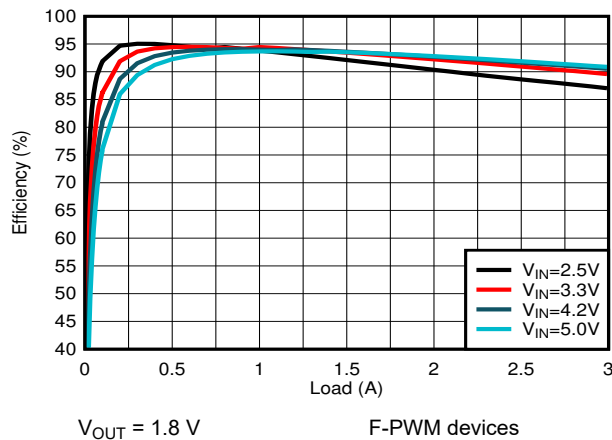
Figure 9-13. PWM Efficiency
