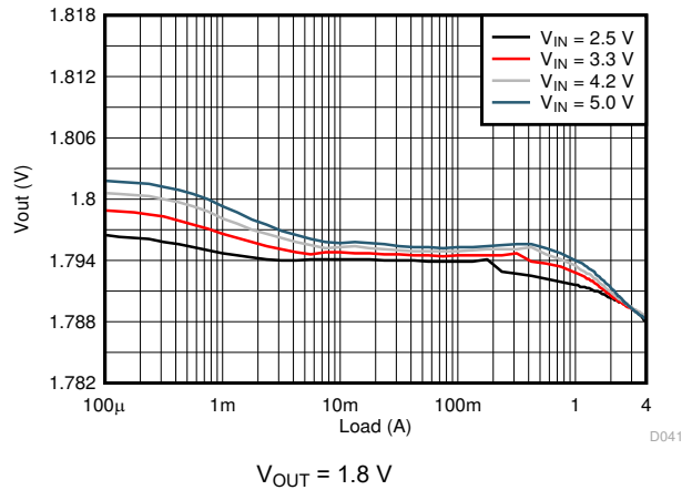
Figure 9-12. Load Regulation
