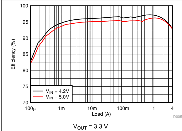
Figure 9-19. Efficiency
