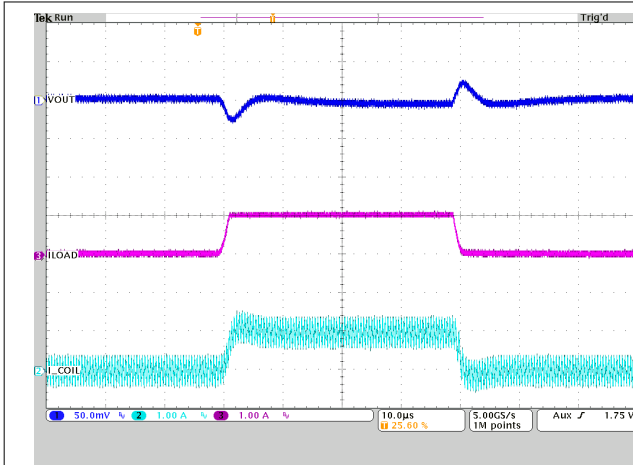
I_{OUT} = 0.05 \text{ A to } 1\text{ A} TPS62825A and TPS62826A
