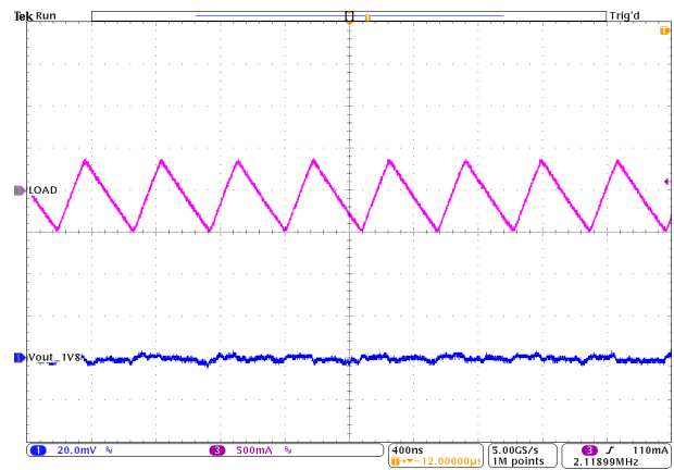
No load TPS6282xA
