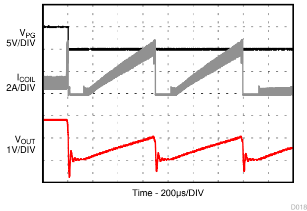
I_{OUT} = 1 \text{ A} TPS62825 and TPS62826
