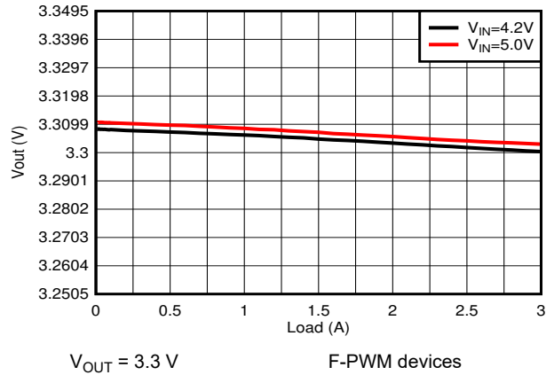
Figure 9-22. Load Regulation
