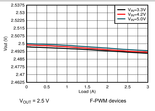
Figure 9-18. Load Regulation
