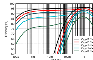
Efficiency at V_{IN} = 5 V
