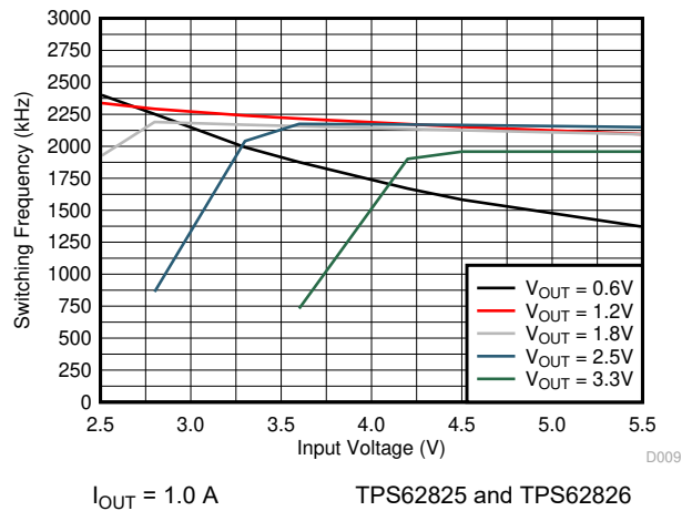
Figure 9-24. Switching Frequency
