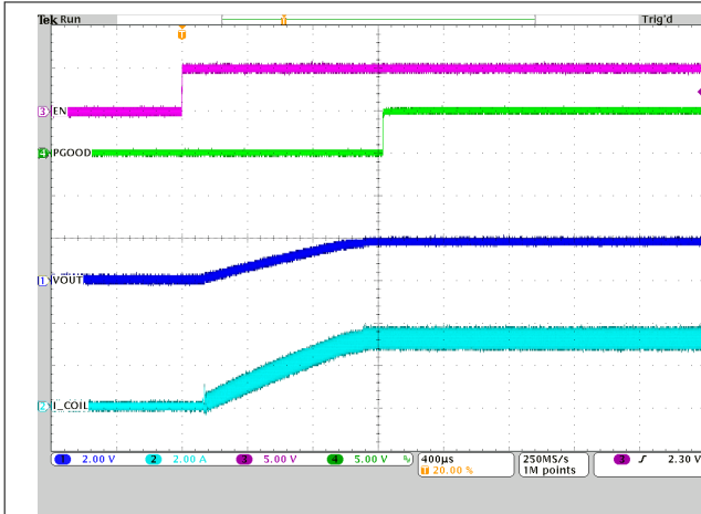
Load = 0.6 \Omega TPS6282xA
