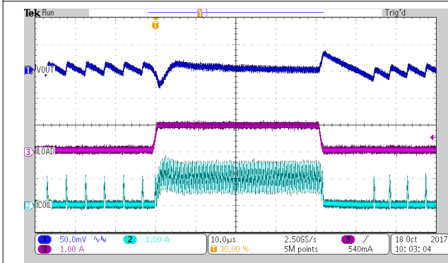
I_{OUT} = 0.05 \text{ A to } 1 \text{ A} TPS62825 and TPS62826
