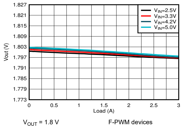
Figure 9-14. Load Regulation
