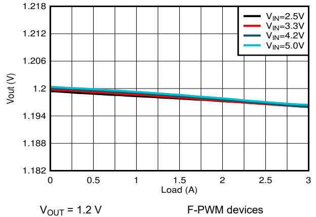
Figure 9-10. Load Regulation
