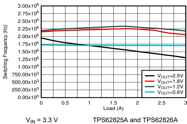
Figure 9-25. Switching Frequency
