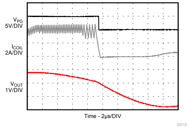
I_{OUT} = 1 \text{ A} TPS62825 and TPS62826
