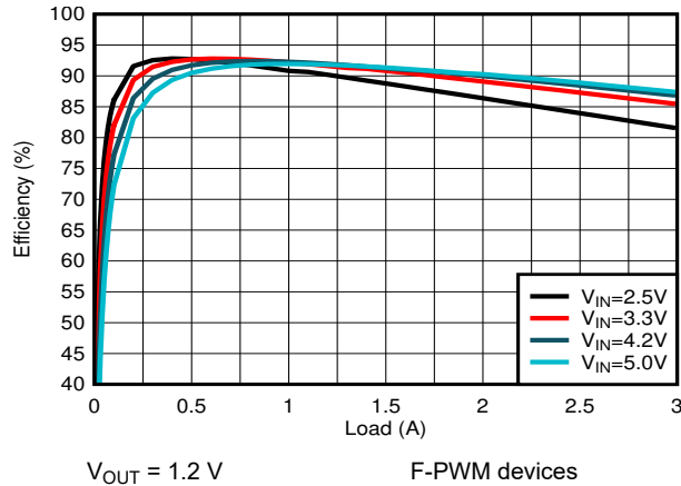
Figure 9-9. PWM Efficiency
