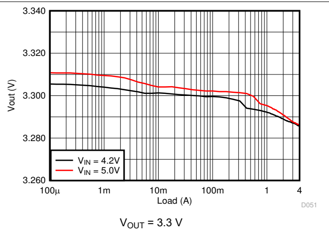
Figure 9-20. Load Regulation
