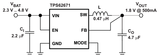
Figure 2. Smallest Solution Size Application
