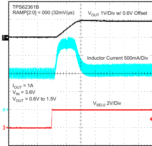
OUTPUT VOLTAGE RAMP CONTROL I_{OUT} = 1A
