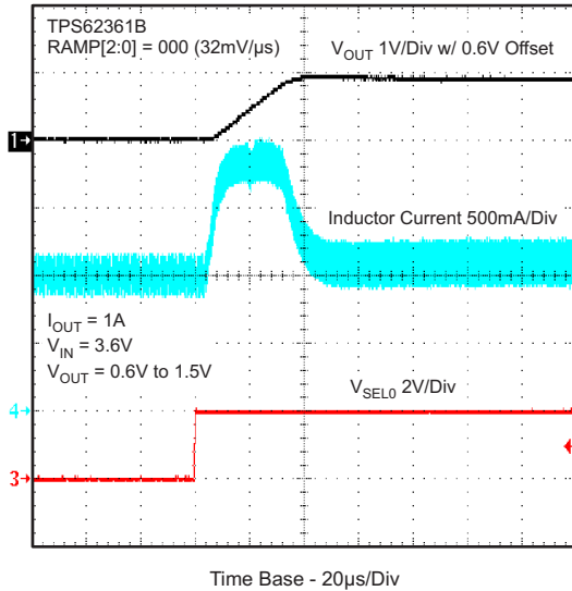
OUTPUT VOLTAGE RAMP CONTROL I_{OUT} = 1A
