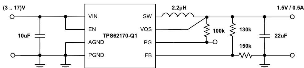
Figure 35. 1.5-V/0.5-A Power Supply
