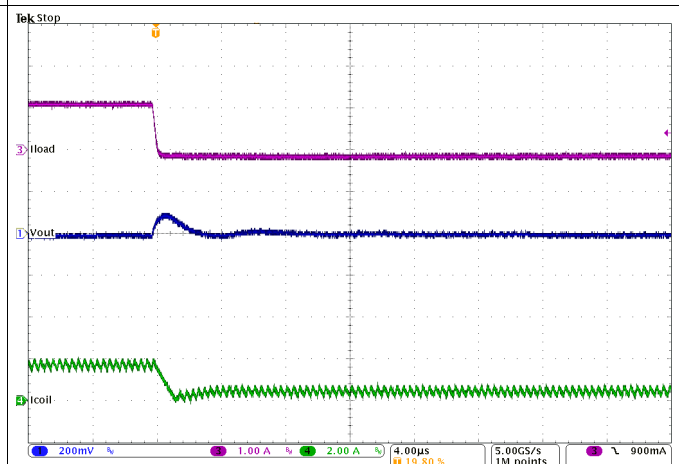
Figure 33. Line Transient Response of Figure 31, Falling Edge
