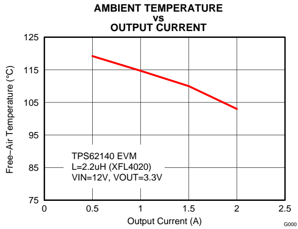
Figure 37. Maximum Ambient Temperature ( f_{SW} = 2.5 MHz)
