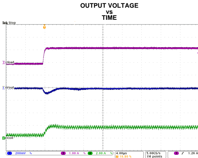
Figure 31. Line Transient Response of Figure 30, Rising Edge
