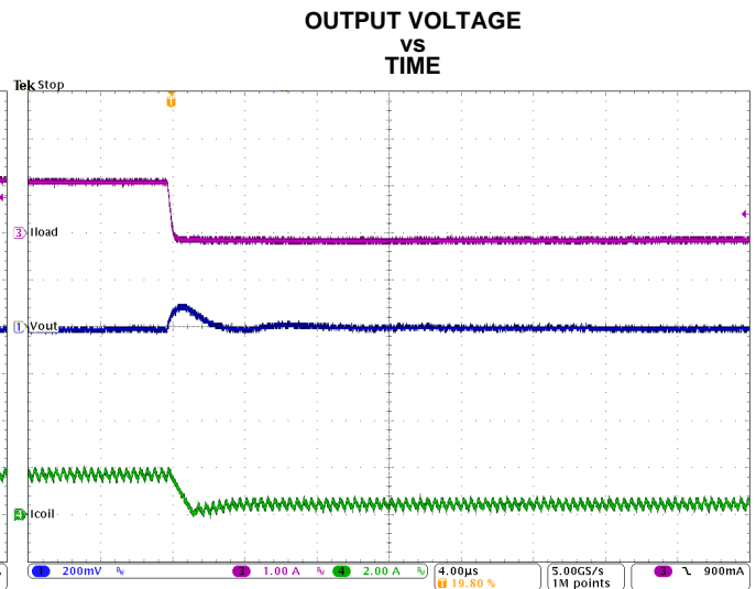
Figure 32. Line Transient Response of Figure 30, Falling Edge
