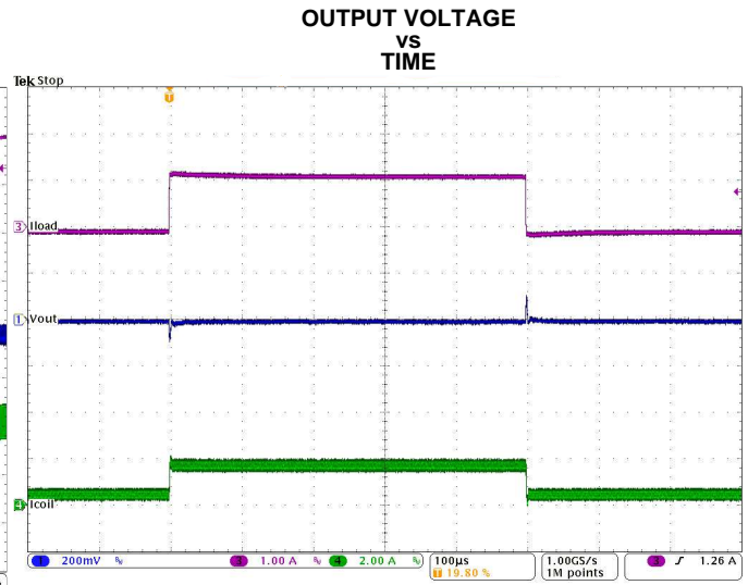
Figure 30. Load Transient Response ( I_{OUT} = 0.5\text{ to }2\text{ to }0.5\text{ A} , V_{IN} = 12\text{ V} , V_{OUT} = 3.3\text{ V} )
