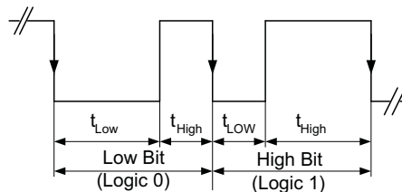
Figure 16. EasyScale™ — Bit Coding
