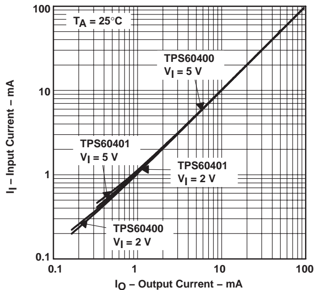
TPS60400, TPS60401 INPUT CURRENT vs OUTPUT CURRENT
