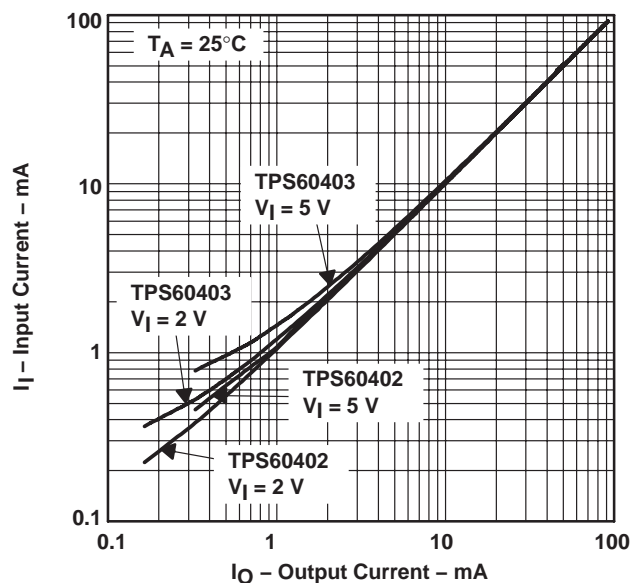
TPS60402, TPS60403 INPUT CURRENT vs OUTPUT CURRENT
