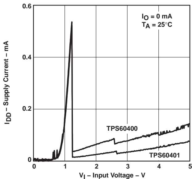
TPS60400, TPS60401 SUPPLY CURRENT vs INPUT VOLTAGE
