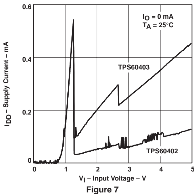
TPS60402, TPS60403 SUPPLY CURRENT vs INPUT VOLTAGE
