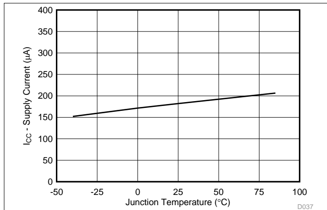
Figure 10. Supply Current vs Junction Temperature
