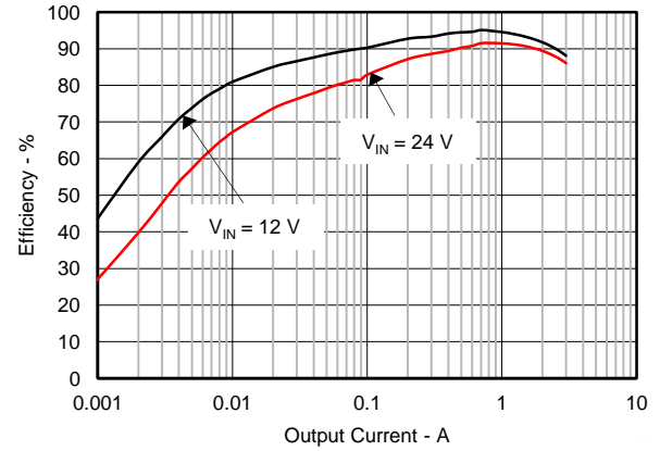
Figure 40. TPS54336 Low Current Efficiency
