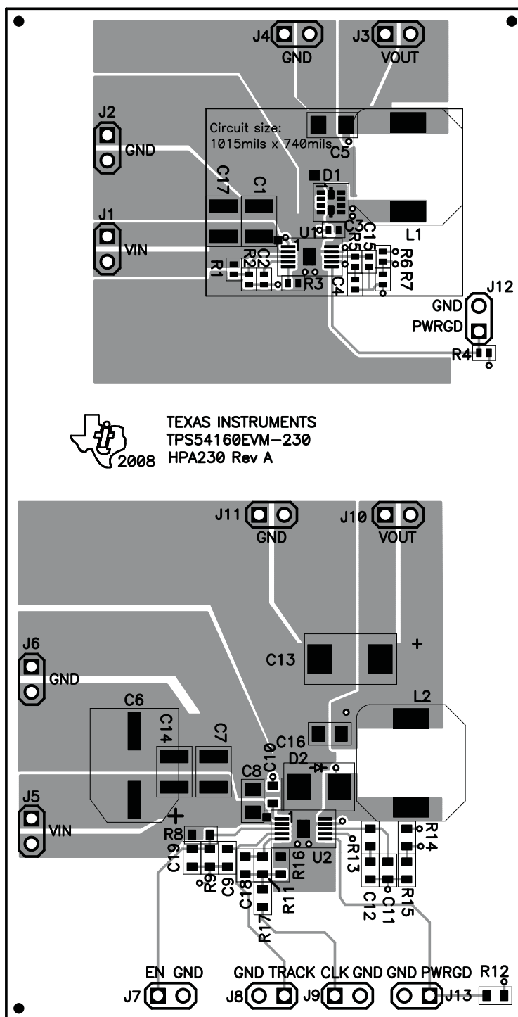
Figure 16. Assembly Layer
