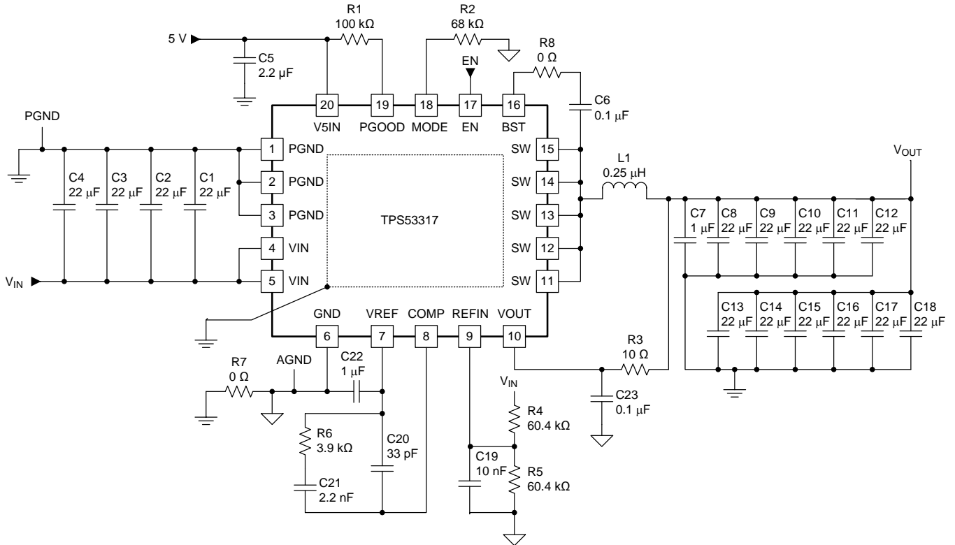
Figure 39. Design Example 2 Schematic: DDR3 Application
