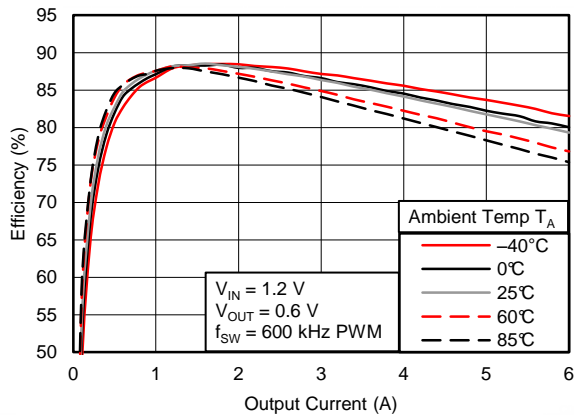
Figure 16. Efficiency vs. Output Current, V_{IN} = 1.2\text{ V}
