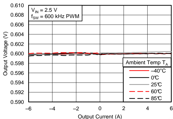
Figure 24. Load Regulation, V_{IN} = 2.5\text{ V}
