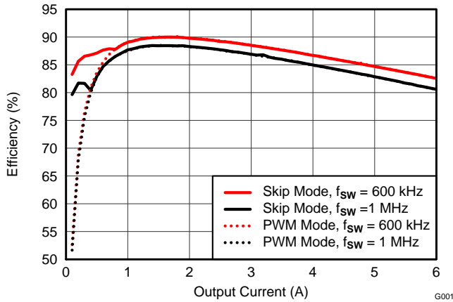
Figure 28. Efficiency vs Output Current V_{IN} = 1.5\text{ V} , V_{OUT} = 0.75\text{ V}
