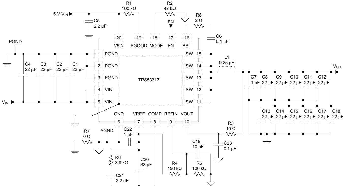
Figure 40. Design Example 3 Schematic: Non-Tracking POL Application
