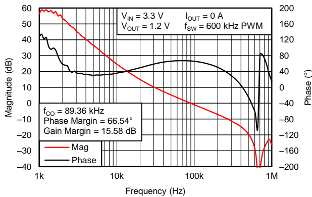
Figure 41. Bode Plot No Load
