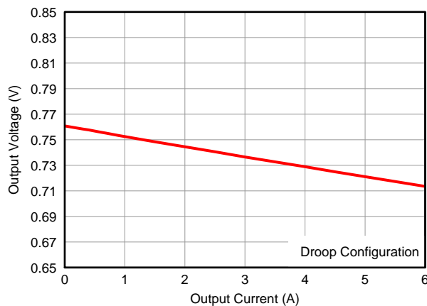
Figure 9. Load Regulation for 1.5-V Input, 0.75-V Output (Droop Configuration)
