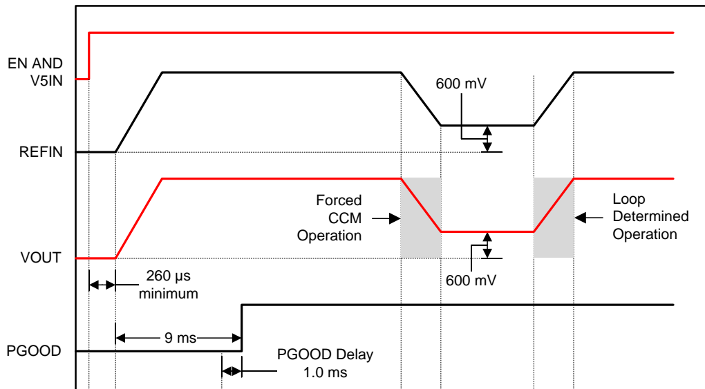
Figure 15. Tracking Startup Timing
