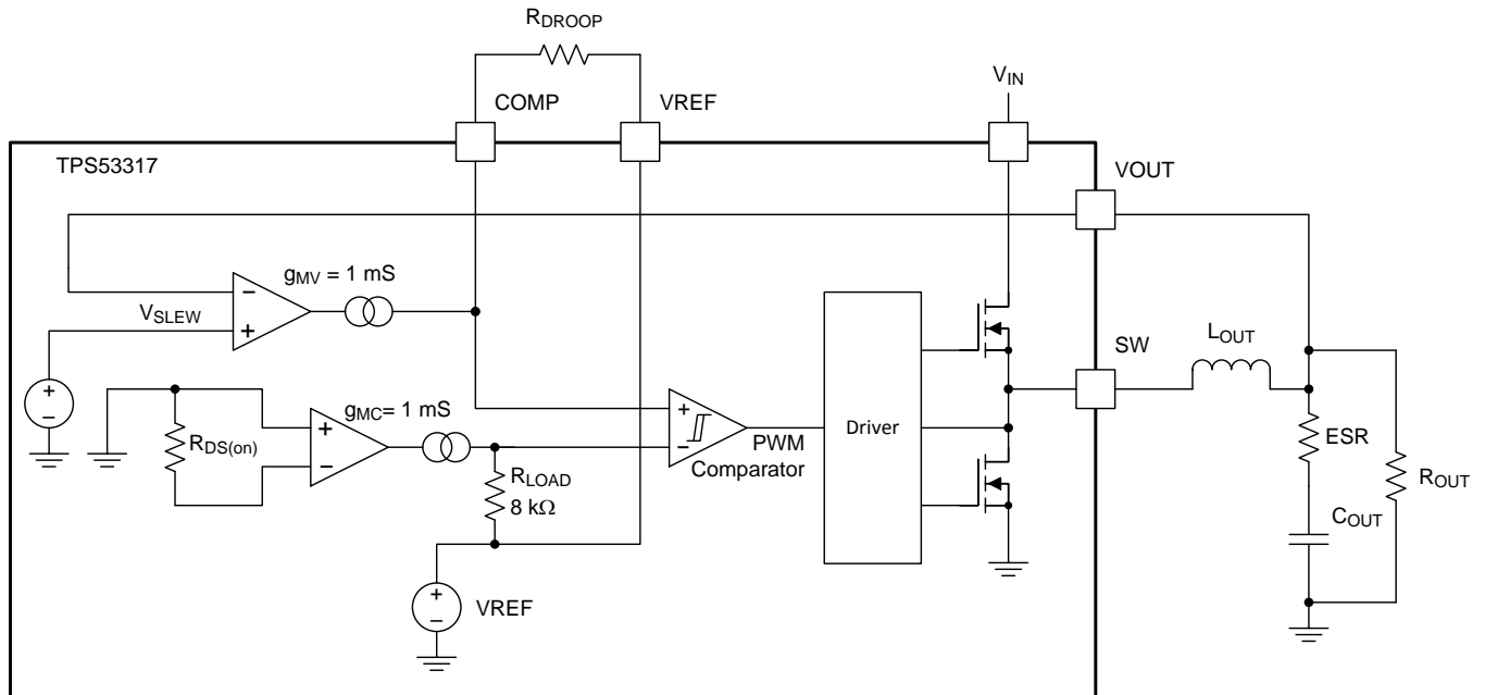
Figure 7. DROOP Mode Basic Implementation
