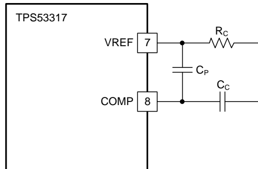
Figure 31. Compensation Network Circuit
