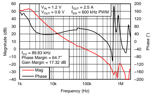
Figure 36. Bode Plot, Full Load
