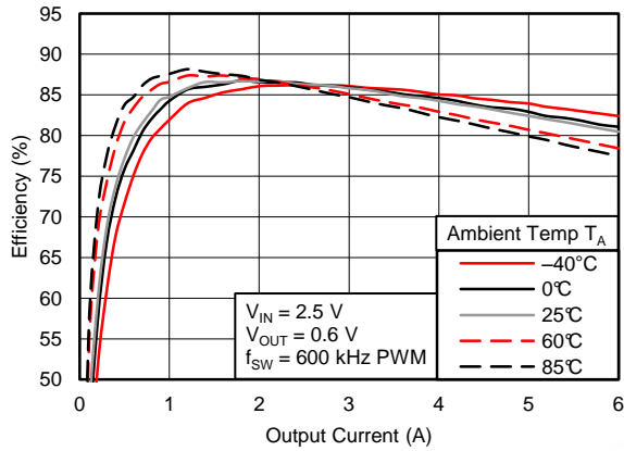
Figure 18. Efficiency vs. Output Current, V_{IN} = 2.5\text{ V}
