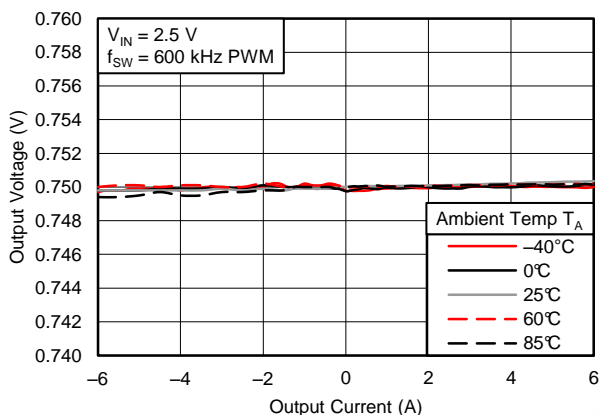
Figure 25. Load Regulation, V_{IN} = 2.5\text{ V}
