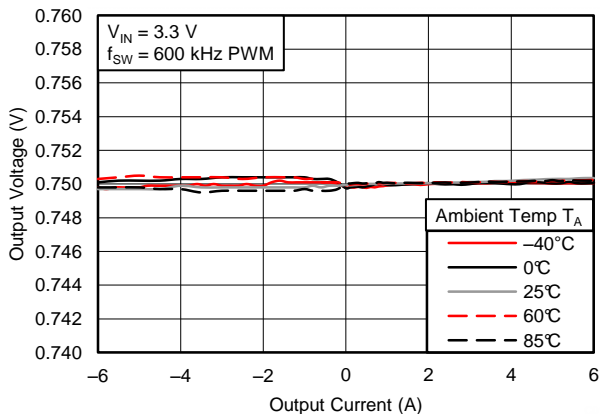
Figure 27. Load Regulation, V_{IN} = 3.3\text{ V}
