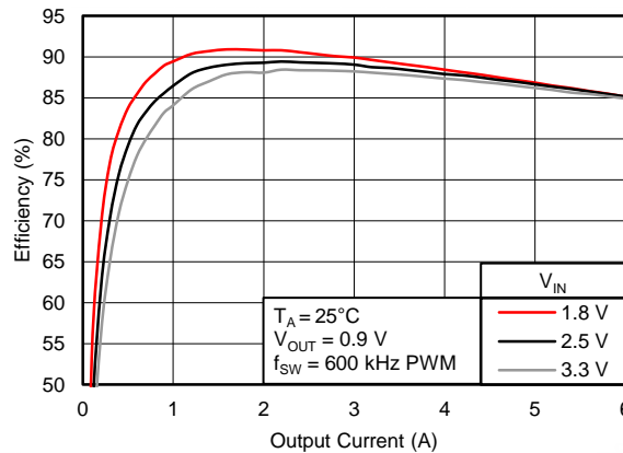
Figure 30. Efficiency vs. Output Current, V_{OUT} = 0.9\text{ V}
