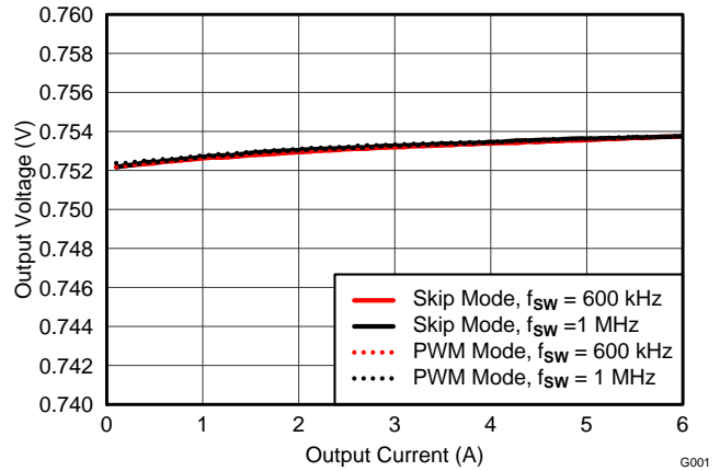
Figure 29. Load Regulation V_{IN} = 1.5\text{ V} , V_{OUT} = 0.75\text{ V}
