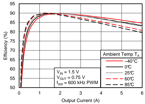
Figure 17. Efficiency vs. Output Current, V_{IN} = 1.5\text{ V}
