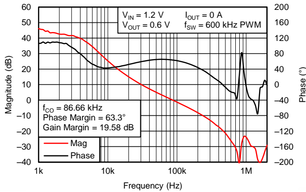
Figure 35. Bode Plot, No Load
