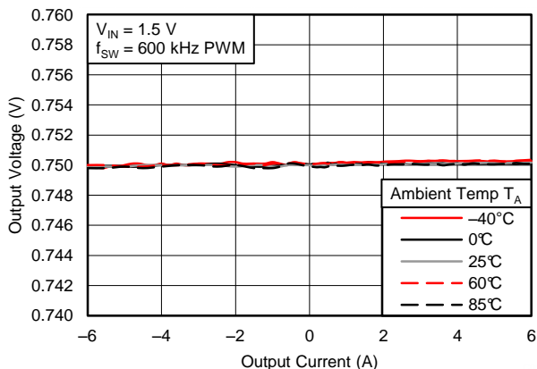
Figure 23. Load Regulation, V_{IN} = 1.5\text{ V}
