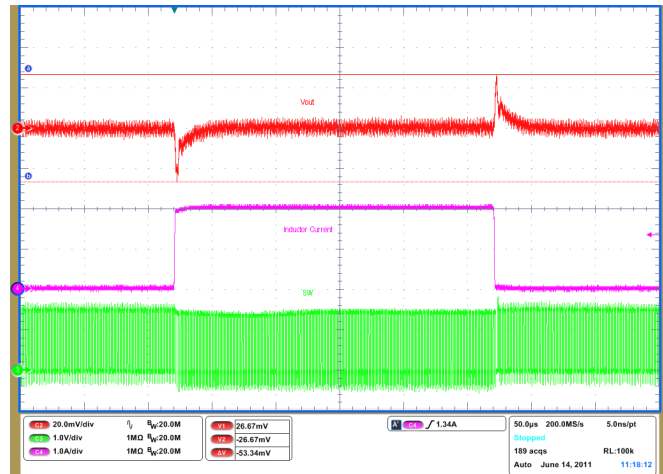
Figure 6. Non-Droop Configuration Transient Response CH 2: V_{OUT} (20 mV/div) CH 4: I_{OUT} (1 A/div) CH 3: SW (1 V/div)
