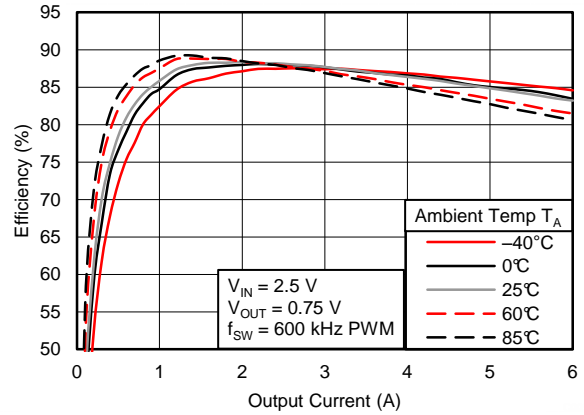
Figure 19. Efficiency vs. Output Current, V_{IN} = 2.5\text{ V}
