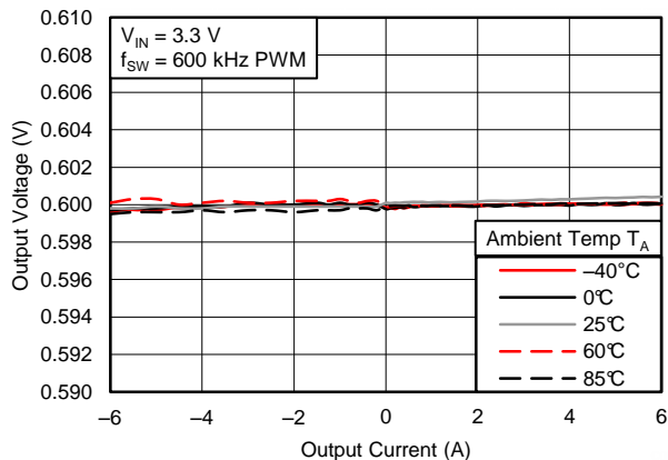
Figure 26. Load Regulation, V_{IN} = 3.3\text{ V}
