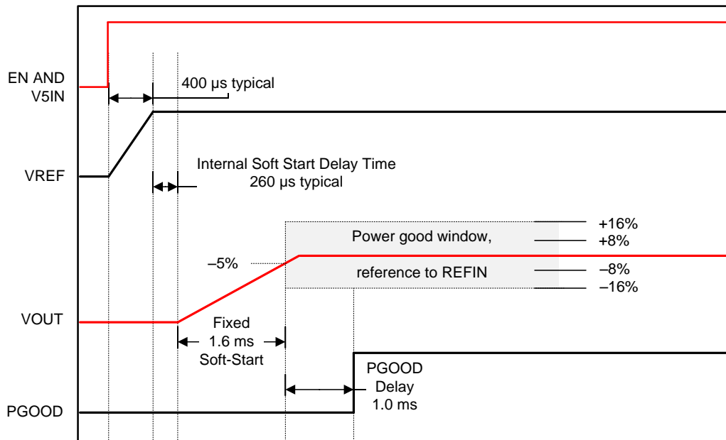
Figure 12. Non-Tracking Startup Timing
