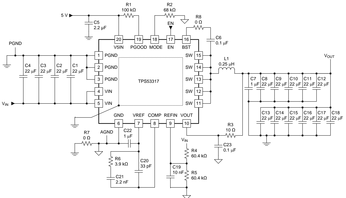
Figure 32. Design Example 1: DDR4 Application Schematic
