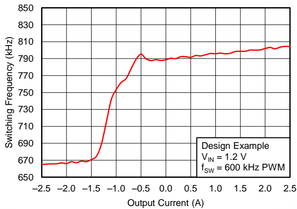
Figure 37. Switching Frequency vs. Load
