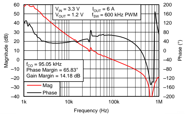
Figure 42. Bode Plot Full Load
