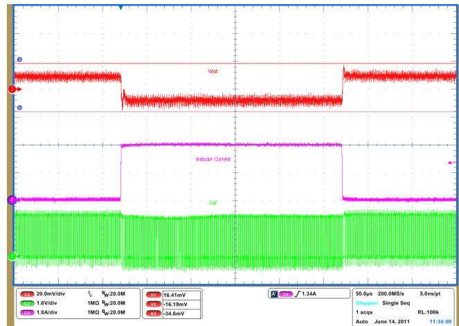
Figure 10. Droop Configuration Transient Response CH 2: V OUT (20 mV/div) CH 4: I OUT (1 A/div) CH 3: SW (1 V/div)
