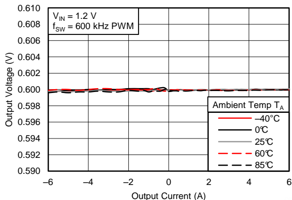
Figure 22. Load Regulation, V_{IN} = 1.2\text{ V}
