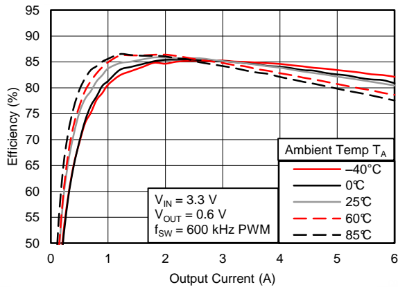
Figure 20. Efficiency vs. Output Current, V_{IN} = 3.3\text{ V}
