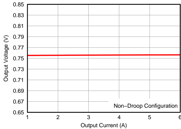
Figure 5. Load Regulation for 1.5-V Input, 0.75-V Output (Non-Droop Configuration)
