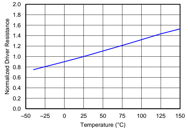
Figure 12. Gate Driver Output Resistance vs Temperature
