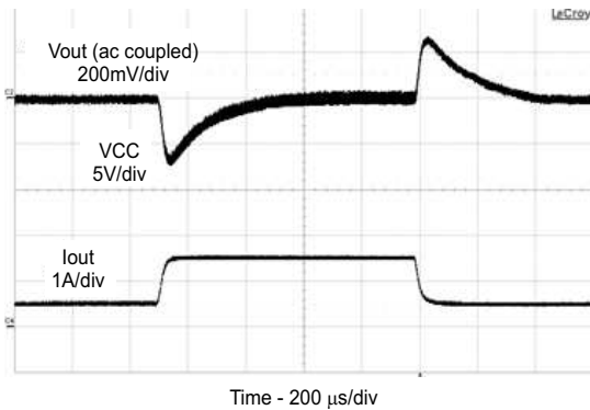
Figure 22. Load Transient
