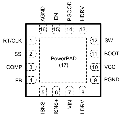
WQFN-16 PACKAGE (TOP VIEW)
