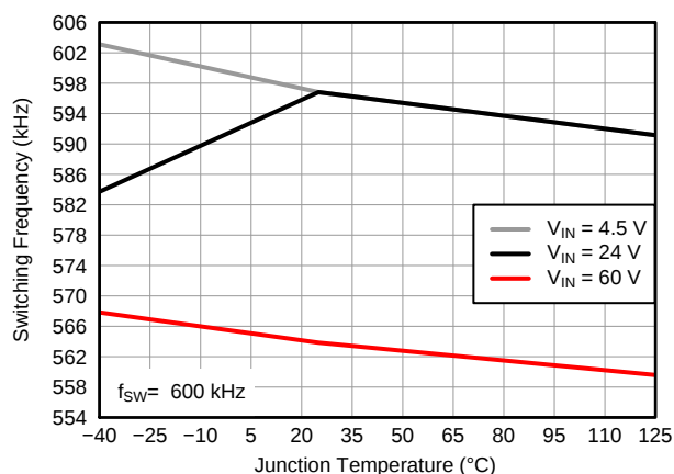
Figure 4. Switching Frequency vs. Junction Temperature (fsw = 600 kHz)
