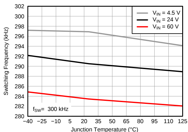
Figure 3. Switching Frequency vs. Junction Temperature (fsw = 300 kHz)
