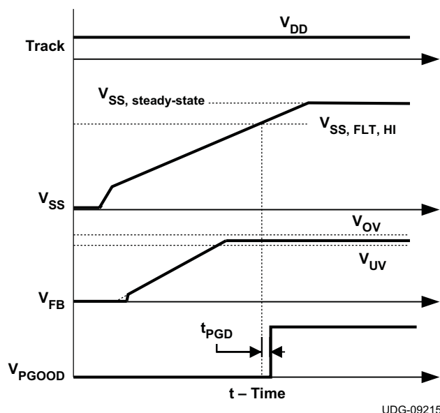
Figure 34. PGOOD Signal
