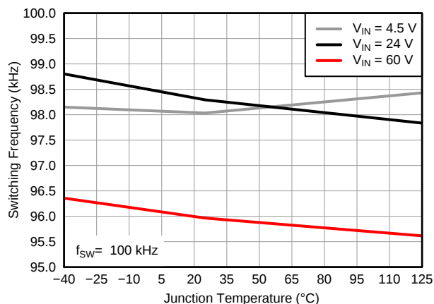
Figure 2. Switching Frequency vs. Junction Temperature (fsw = 100 kHz)
