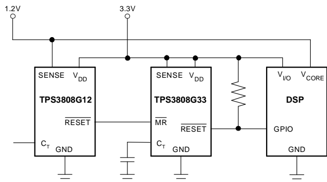
Figure 12. Using MR to Monitor Multiple System Voltages
