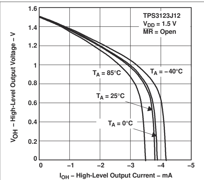
Figure 7-8. HIGH-LEVEL OUTPUT VOLTAGE vs HIGH-LEVEL OUTPUT CURRENT
