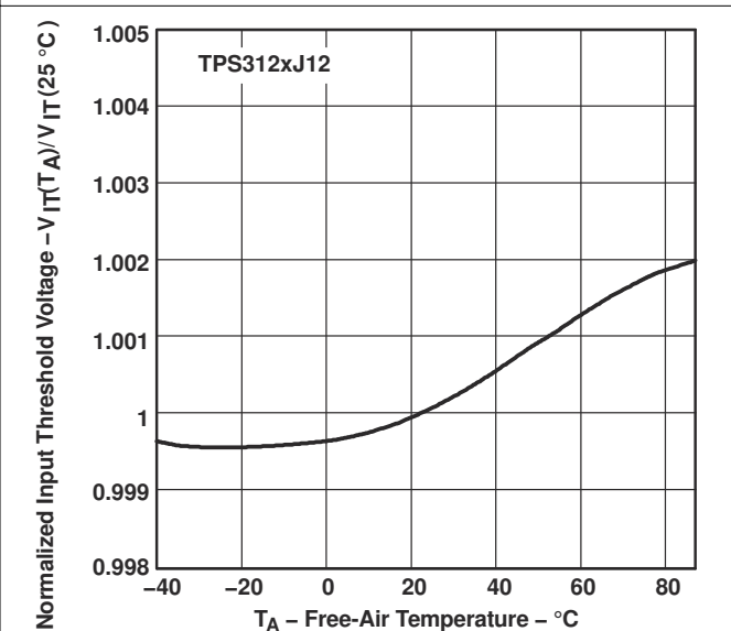
Figure 7-10. NORMALIZED INPUT THRESHOLD VOLTAGE vs FREE-AIR TEMPERATURE
