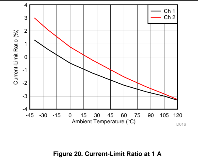
Figure 20. Current-Limit Ratio at 1 A
