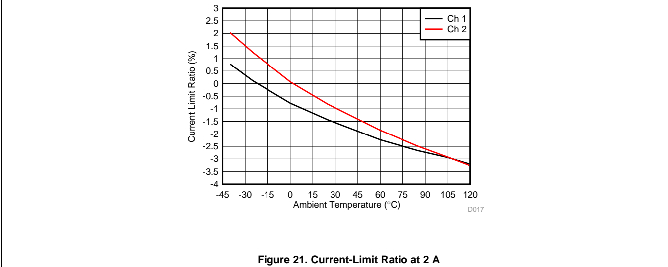
Figure 21. Current-Limit Ratio at 2 A
