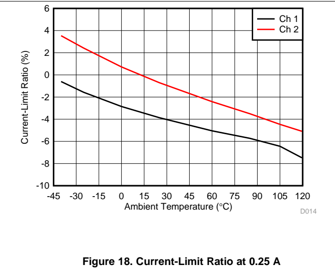
Figure 18. Current-Limit Ratio at 0.25 A
