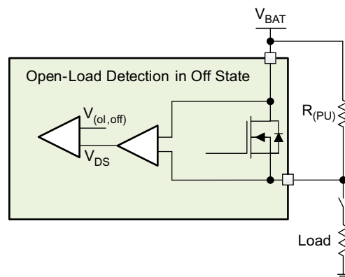
Figure 31. Open-Load Detection in Off-State
