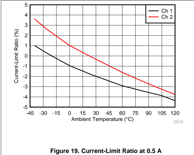
Figure 19. Current-Limit Ratio at 0.5 A
