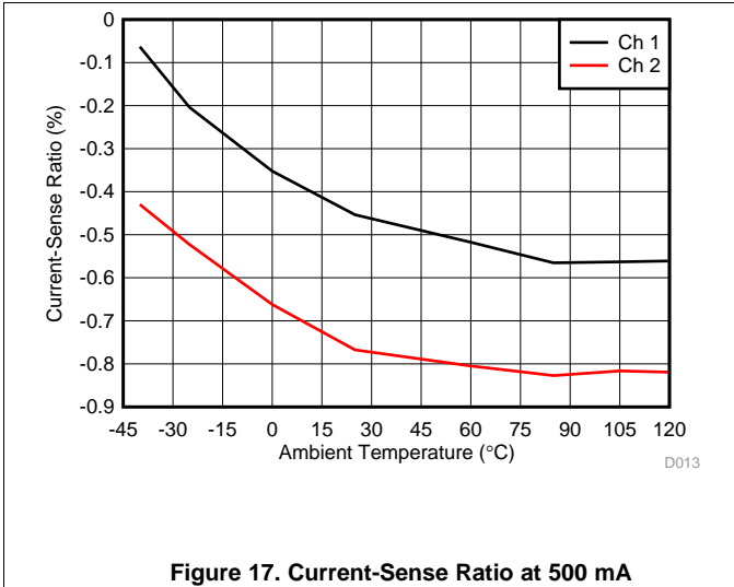
Figure 17. Current-Sense Ratio at 500 mA
