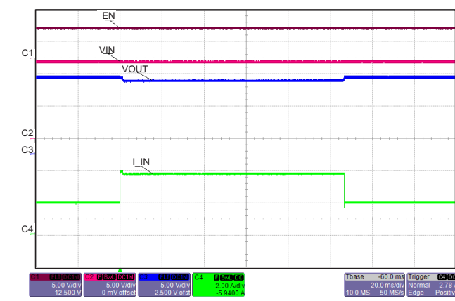
Figure 19. Transient: Output Short Circuit
