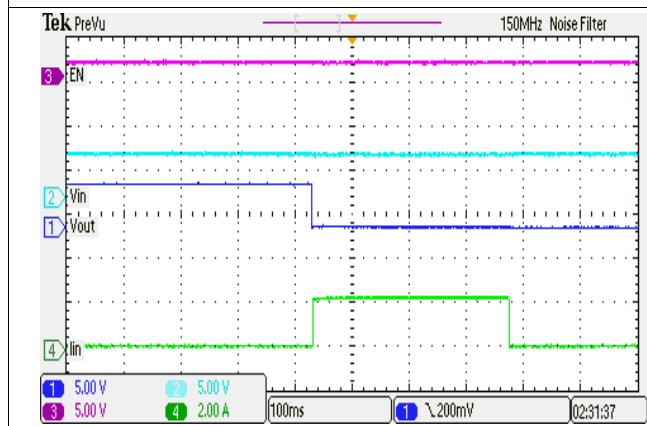
Figure 21. Transient: Overload Current Limit
