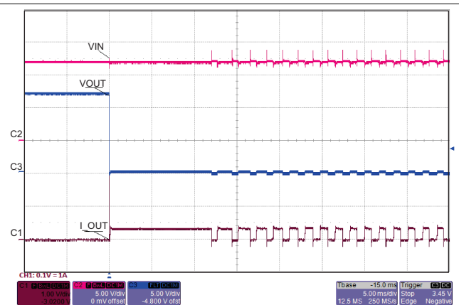
Figure 20. Short Circuit (Zoom): Fast-trip Comparator
