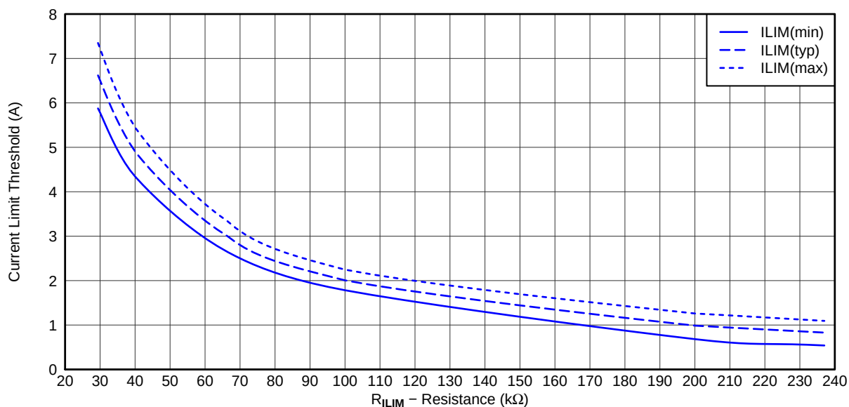
Figure 6. Current Limit Threshold vs. R_{ILIM}
