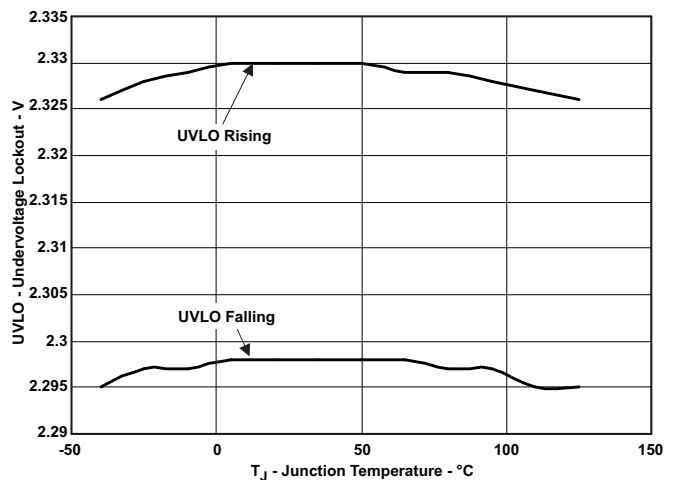
Figure 11. UVLO – Undervoltage Lockout – V
