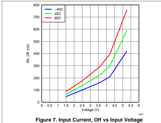
Figure 7. Input Current, Off vs Input Voltage
