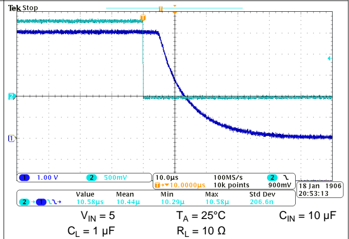
Figure 59. Turn-off Response
