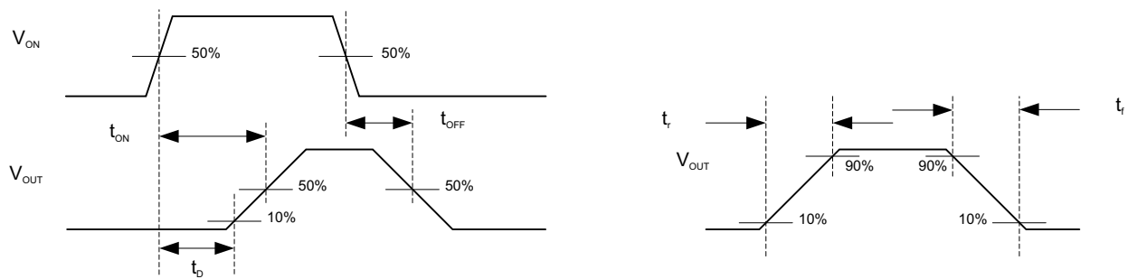
Figure 47. Timing Waveforms
