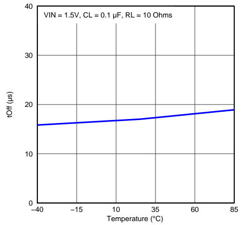
Figure 35. Turn-off Time vs Temperature
