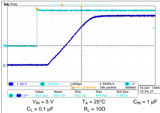
Figure 58. Turn-on Response
