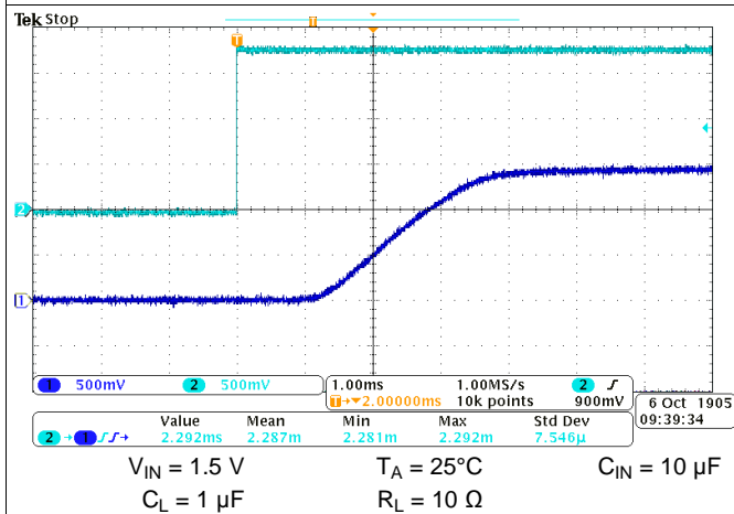
Figure 76. Turn-On Response Time
