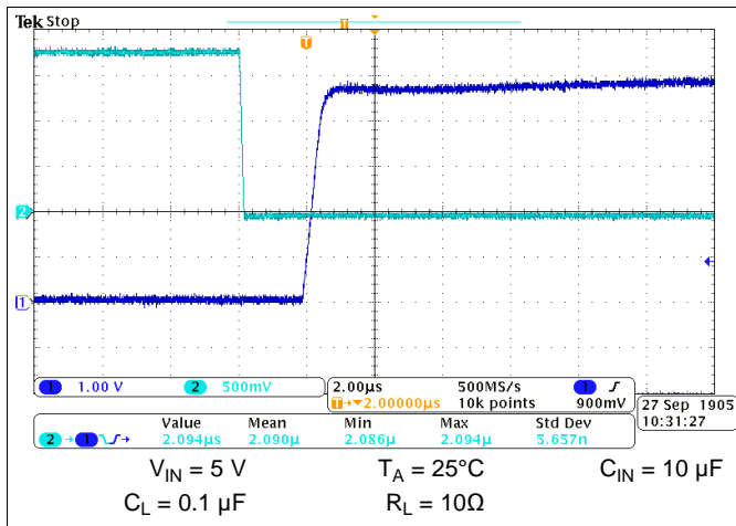
Figure 50. Turn-on Response
