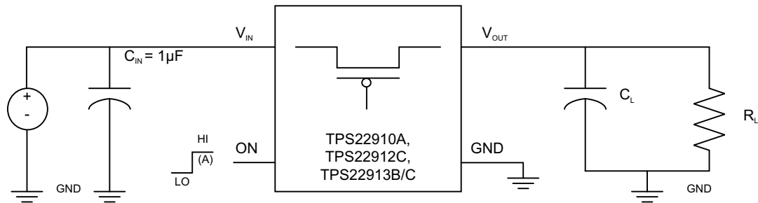
Figure 46. Timing Test Circuit
