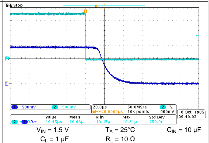
Figure 77. Turn-Off Response Time
