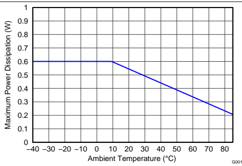
Figure 7. Allowable Power Dissipation
