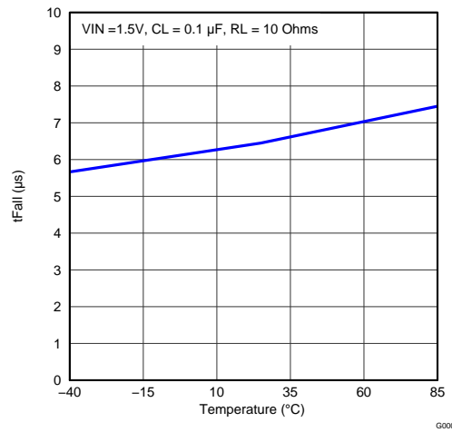
Figure 20. Fall Time vs Temperature
