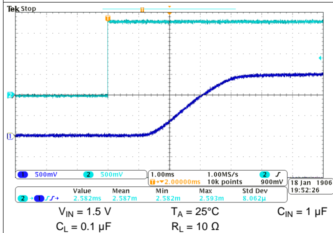
Figure 60. Turn-on Response Time
