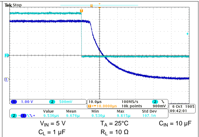
Figure 75. Turn-Off Response Time
