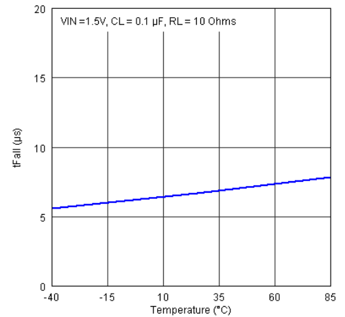
Figure 29. Fall Time vs Temperature
