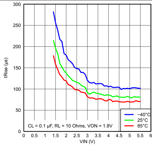
Figure 36. Rise Time vs Input Voltage
