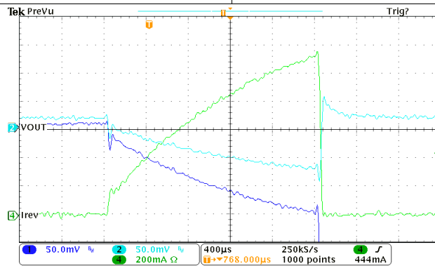
Figure 9. Reverse Current Protection V_{OUT} = 5 \text{ V} (Measured with -5 \text{ V} Offset), Ramping Load on V_{in}
