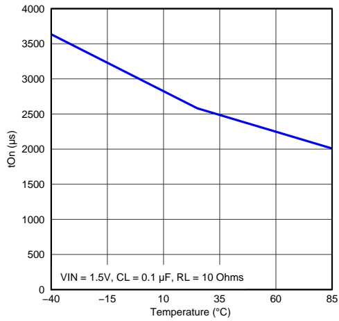
Figure 25. Turn-on Time vs Temperature
