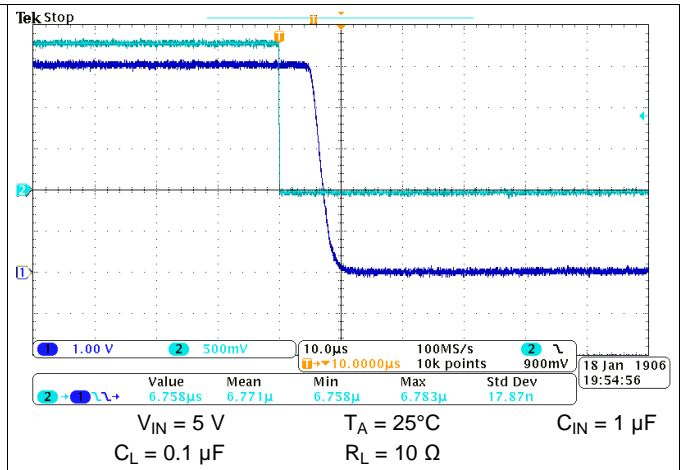
Figure 59. Turn-off Response
