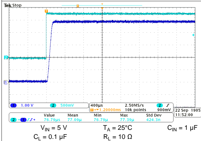
Figure 66. Turn-on Response
