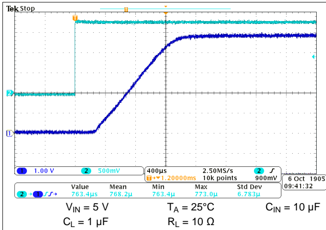
Figure 74. Turn-On Response Time
