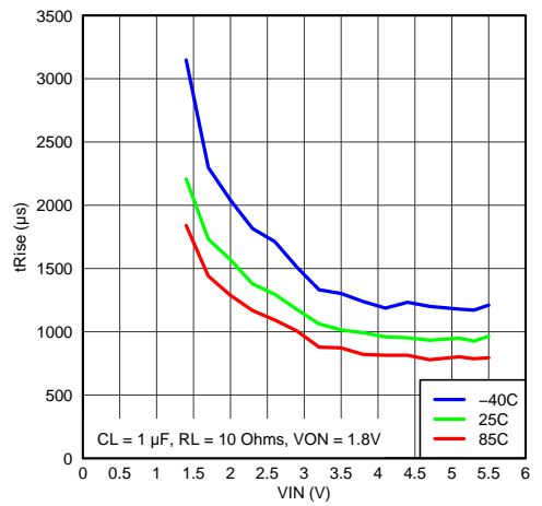
Figure 27. Rise Time vs Input Voltage
