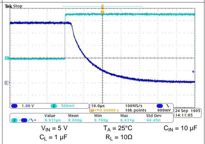
Figure 53. Turn-off Response Time
