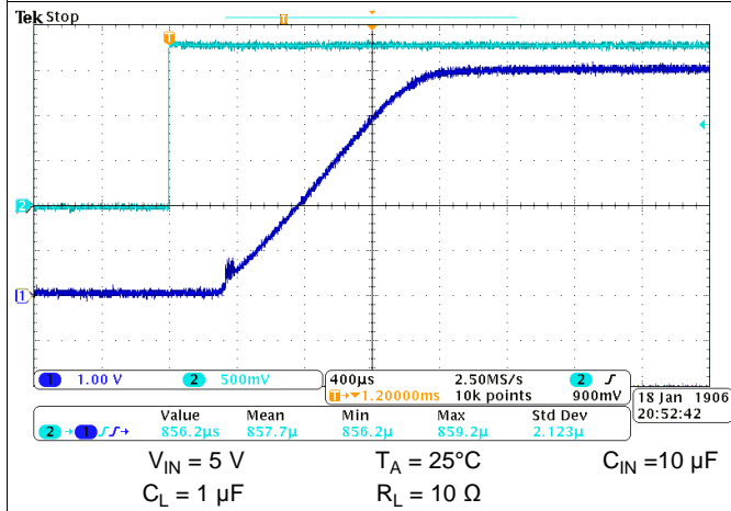
Figure 58. Turn-on Response
