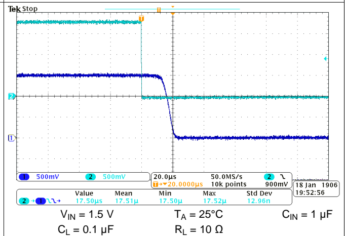
Figure 61. Turn-off Response Time
