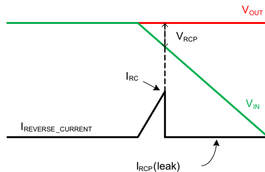
Figure 48. Reverse Current
