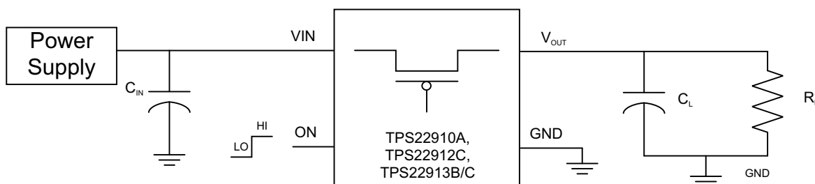
Figure 49. Typical Application
