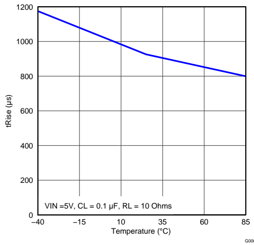
Figure 19. Rise Time vs Temperature
