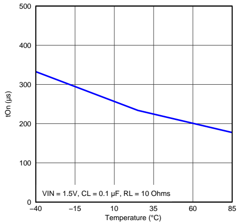
Figure 34. Turn-on Time vs Temperature
