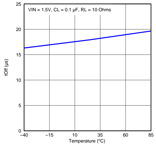
Figure 44. Turn-Off Time vs Temperature
