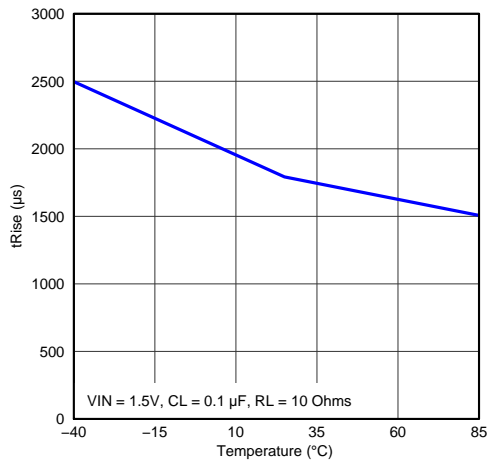
Figure 37. Rise Time vs Temperature
