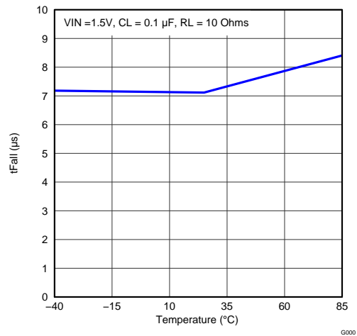
Figure 11. Fall Time vs Temperature
