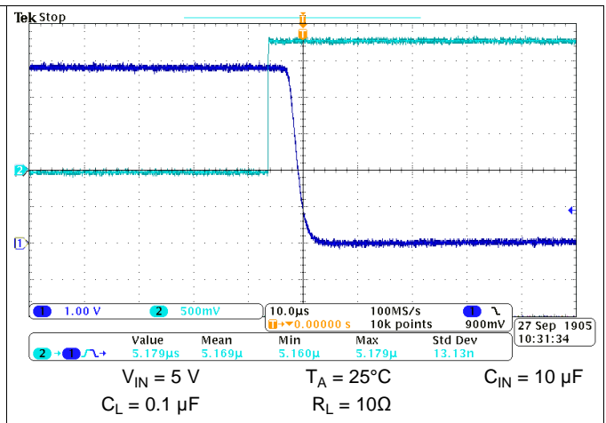
Figure 51. Turn-off Response
