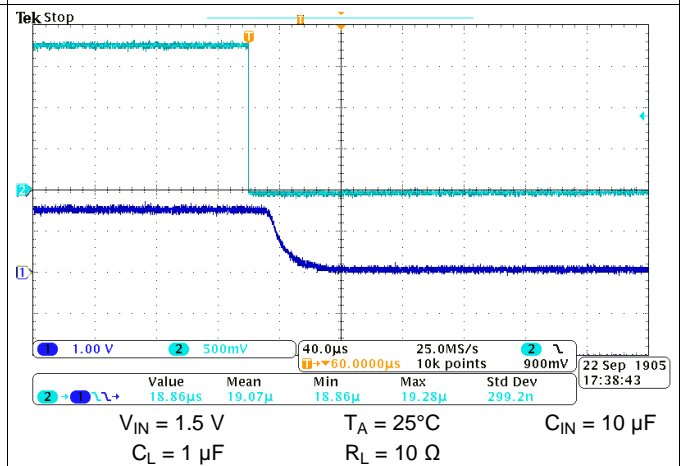
Figure 69. Turn-off Response Time
