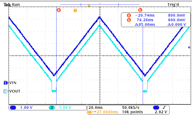
Figure 8. ULVO Response I_{OUT} = -100 \text{ mA}
