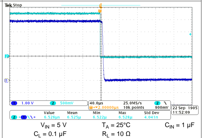
Figure 67. Turn-off Response
