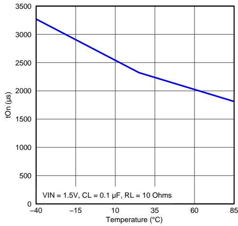
Figure 43. Turn-On Time vs Temperature
