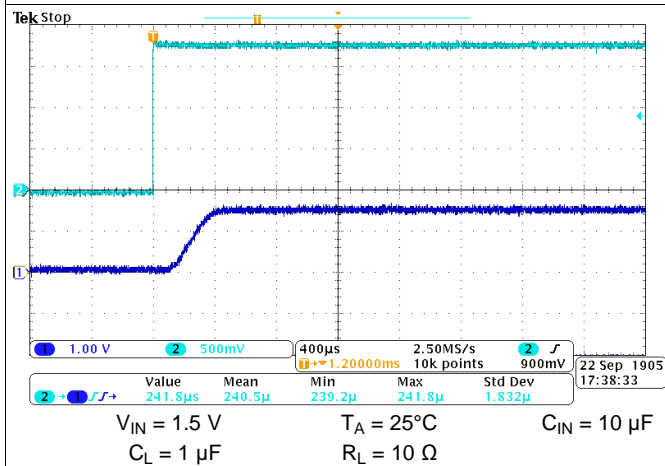
Figure 68. Turn-on Response Time
