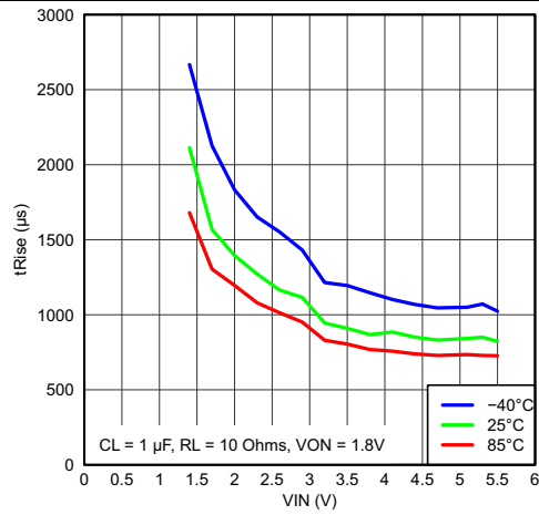
Figure 45. Rise Time vs Input Voltage
