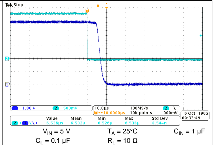
Figure 75. Turn-Off Response Time
