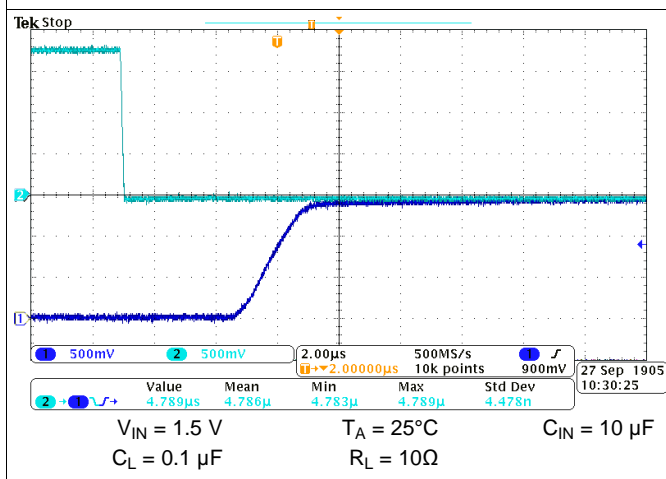
Figure 54. Turn-on Response Time
