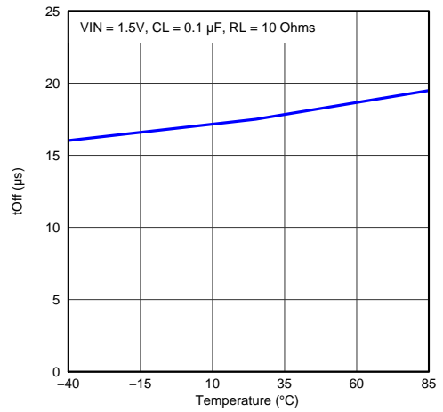
Figure 26. Turn-off Time vs Temperature
