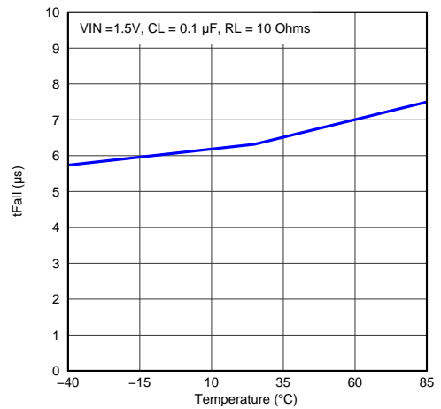
Figure 38. Fall Time vs Temperature
