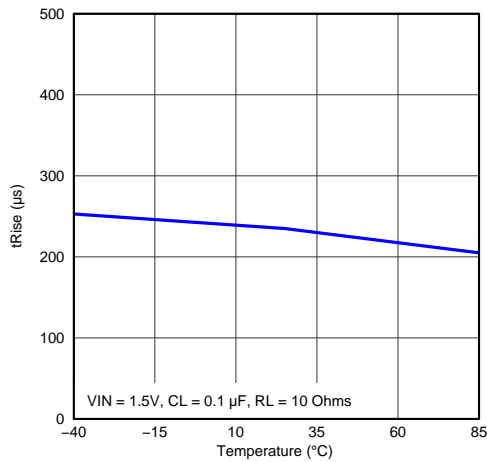
Figure 28. Rise Time vs Temperature
