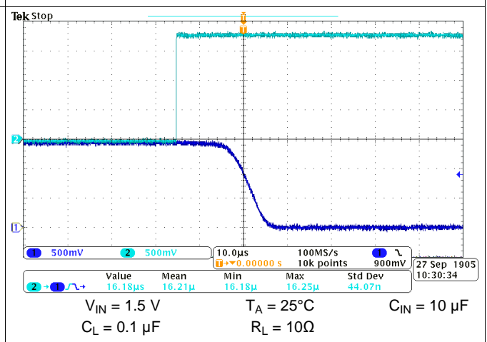
Figure 55. Turn-off Response Time
