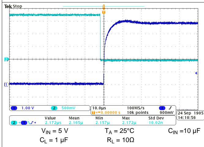
Figure 52. Turn-on Response Time
