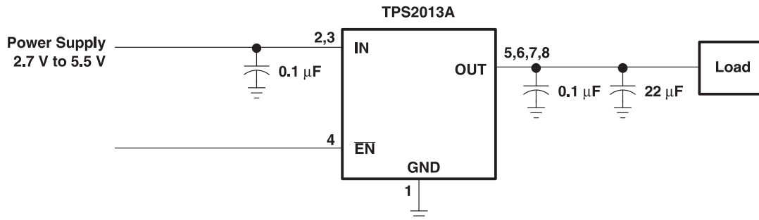
Figure 35. Typical Application
