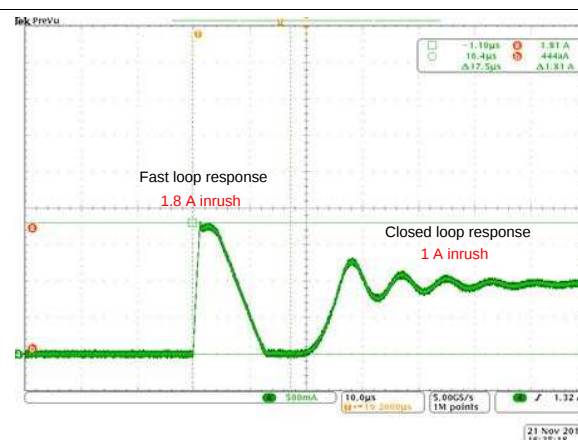
Figure 49. Hard Short to GND Waveform
