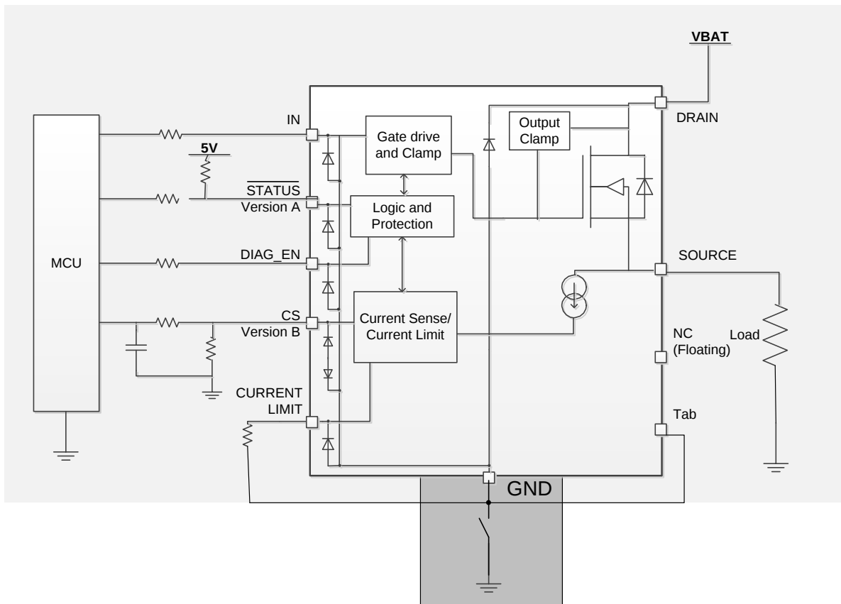
Figure 38. Loss of Device GND
