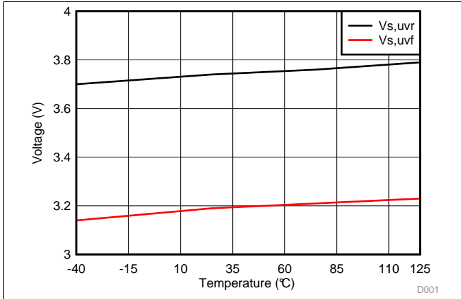
Figure 8. V_{s,uvr} and V_{s,uvf}
