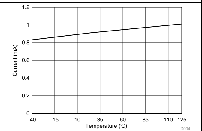
Figure 9. I_{nom} With No Load and 10- \Omega Load
