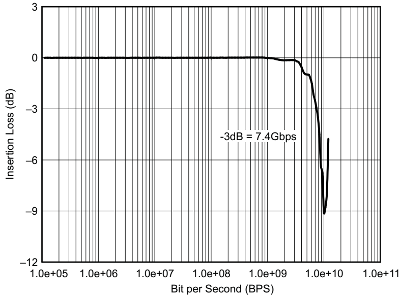
Figure 9. Insertion Loss
